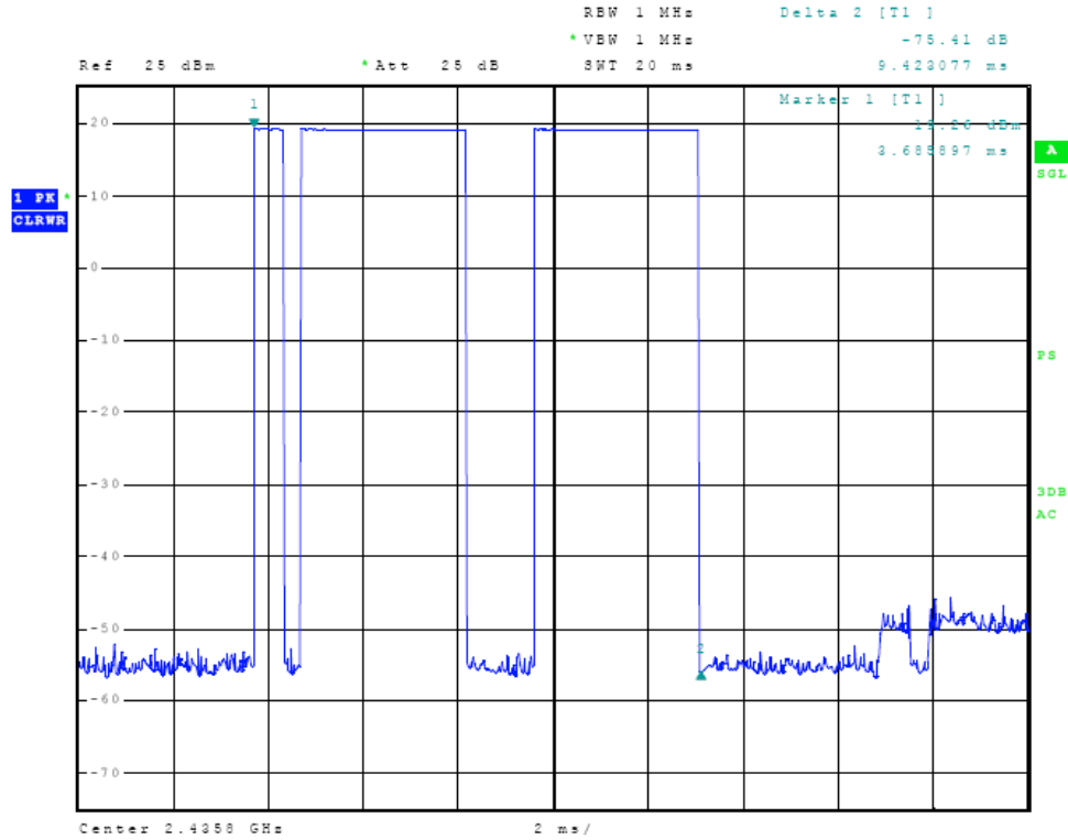
Figure Thirty-two Plot of Dwell time on Channel (79 Hop Set)
