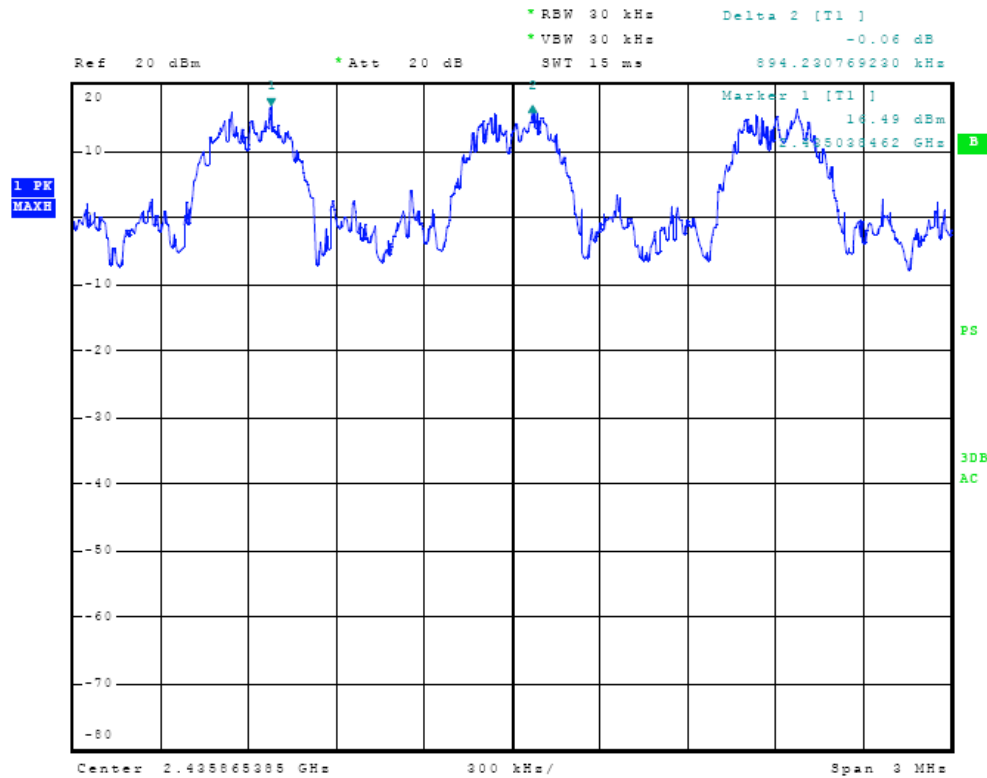
Figure Thirty Plot of Channel Spacing (79 Hop Set)
