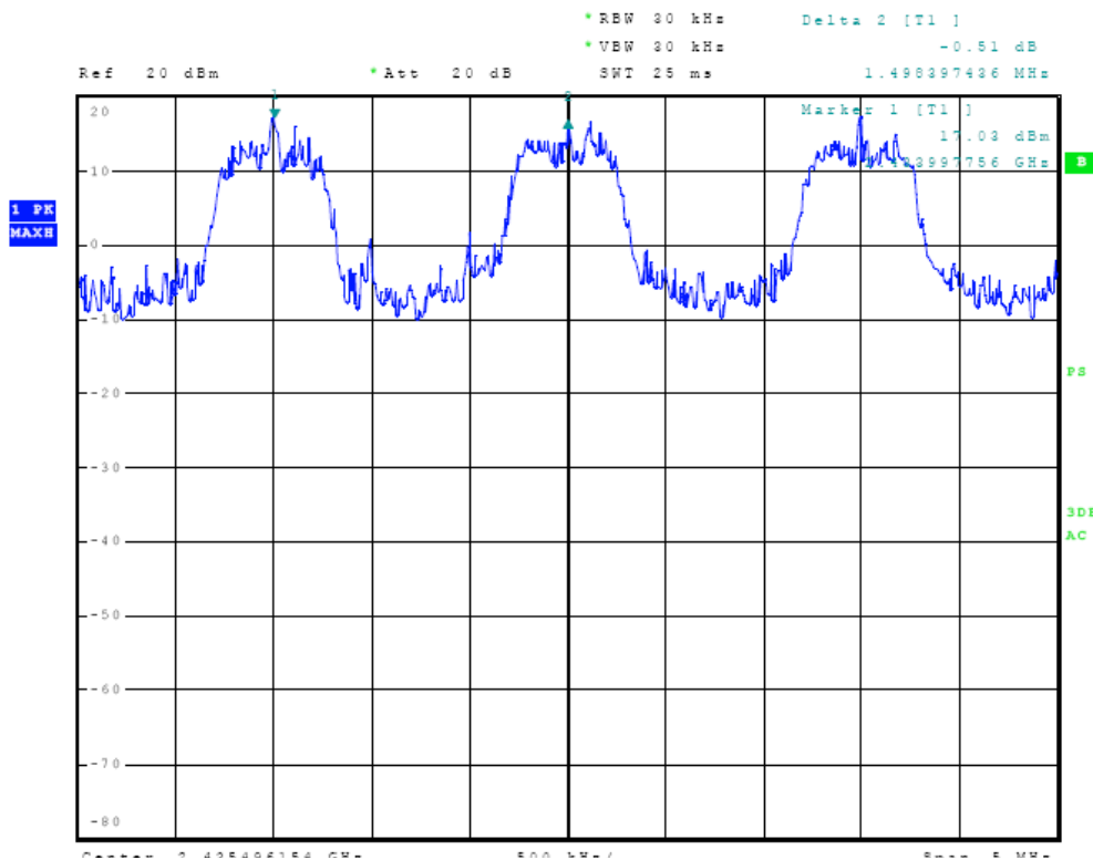
Figure Thirty-one Plot of Channel Spacing (43 Hop Set)
