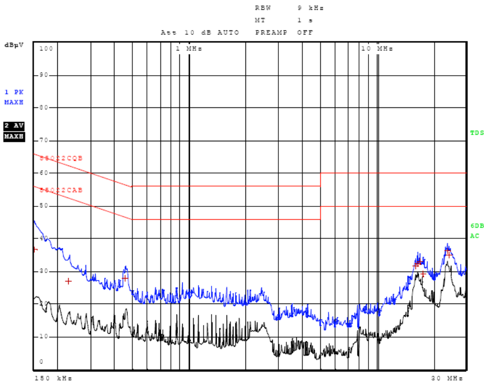
Figure Two AC Line Conducted Emissions Line 2 (configuration 1)
