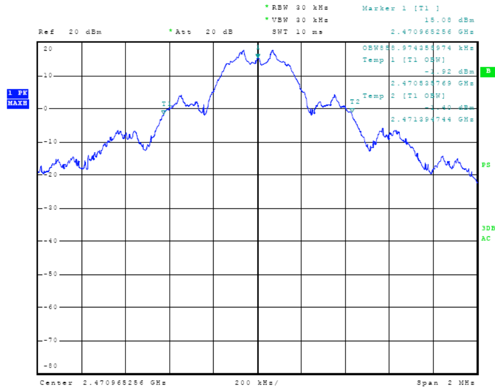
Figure Twenty-six Plot of 20 dB Occupied Bandwidth (79 Hop Set)
