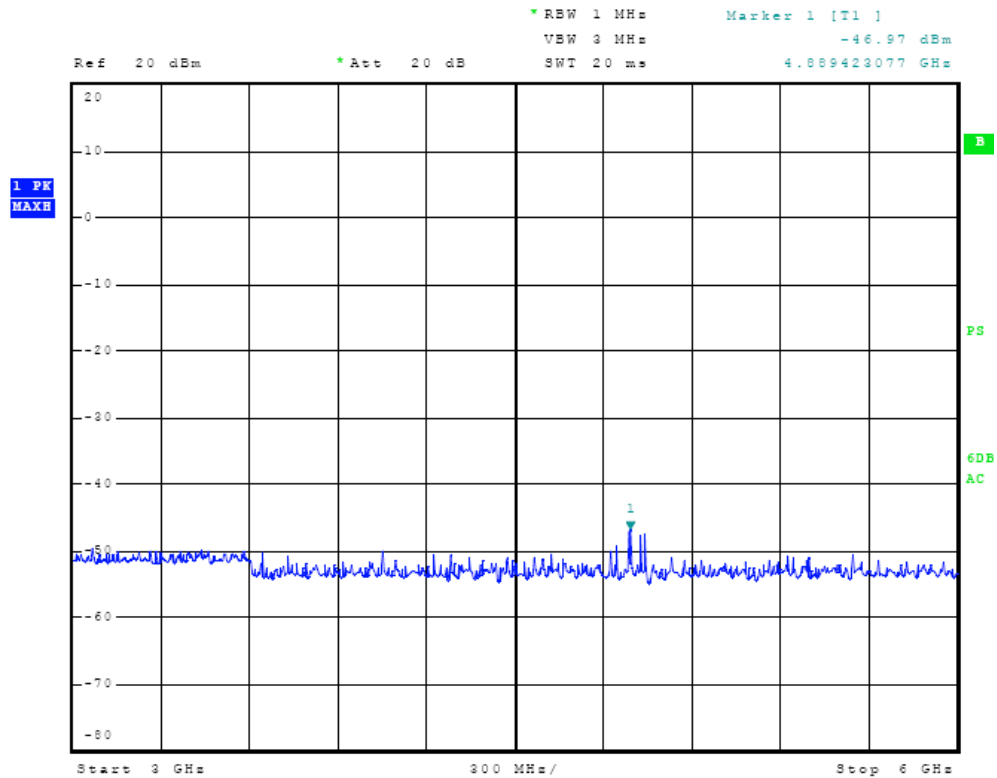
Figure Twenty Plot of Antenna Port Conducted Emissions
