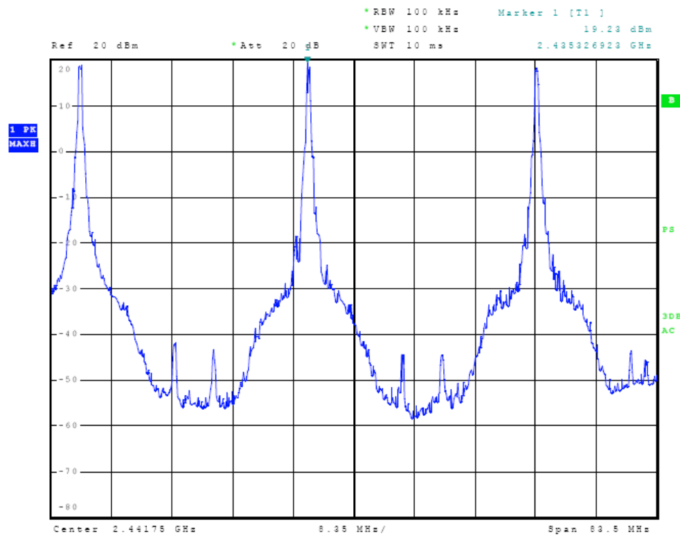
Figure Twenty-three Plot of Operation Across Operational Band (43 Hop Set)
