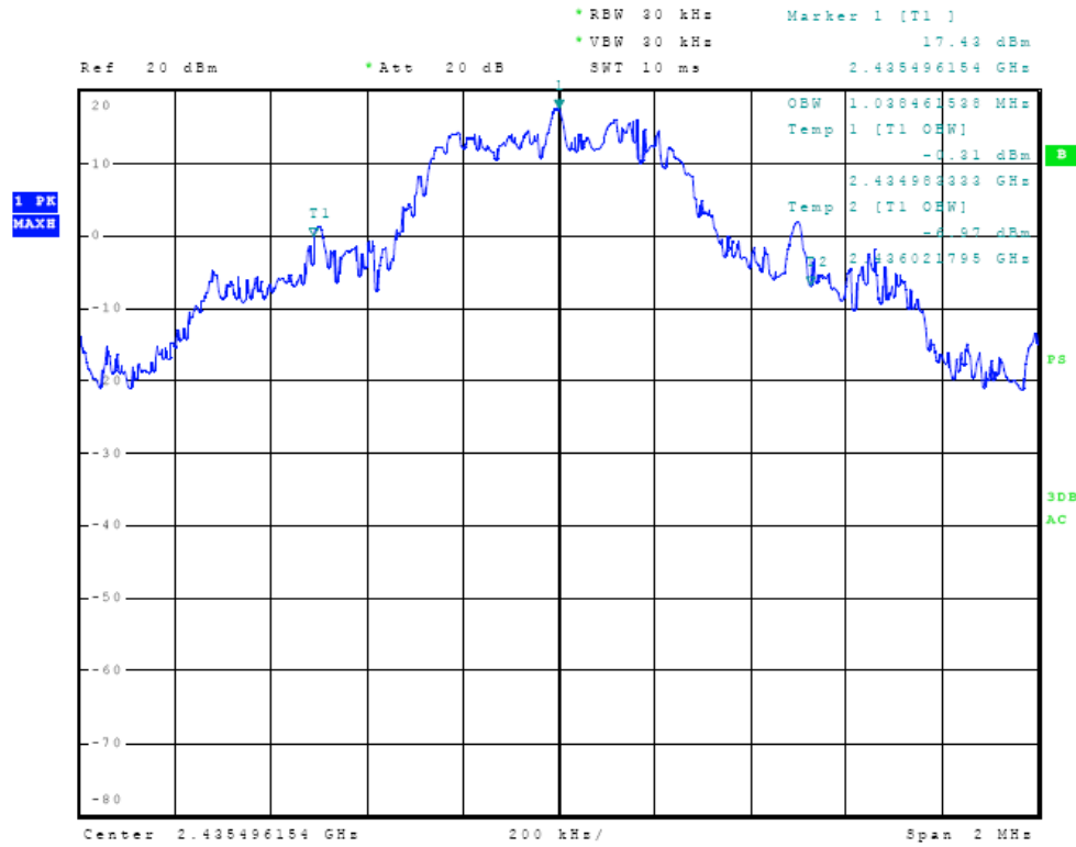
Figure Twenty-eight Plot of 20 dB Occupied Bandwidth (43 Hop Set)
