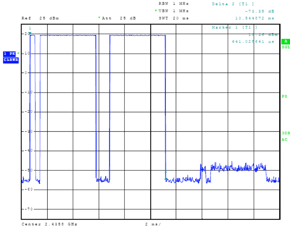
Figure Thirty-four Plot of Plot of Dwell time on Channel (43 Hop Set)
