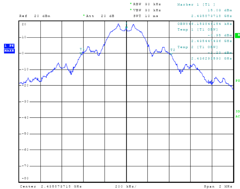
Figure Twenty-five Plot of 20 dB Occupied Bandwidth (79 Hop Set)
