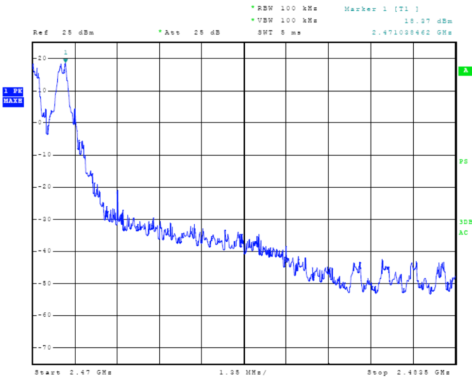
Figure Thirty-seven Plot of High Band Edge (79 Hop Set)
