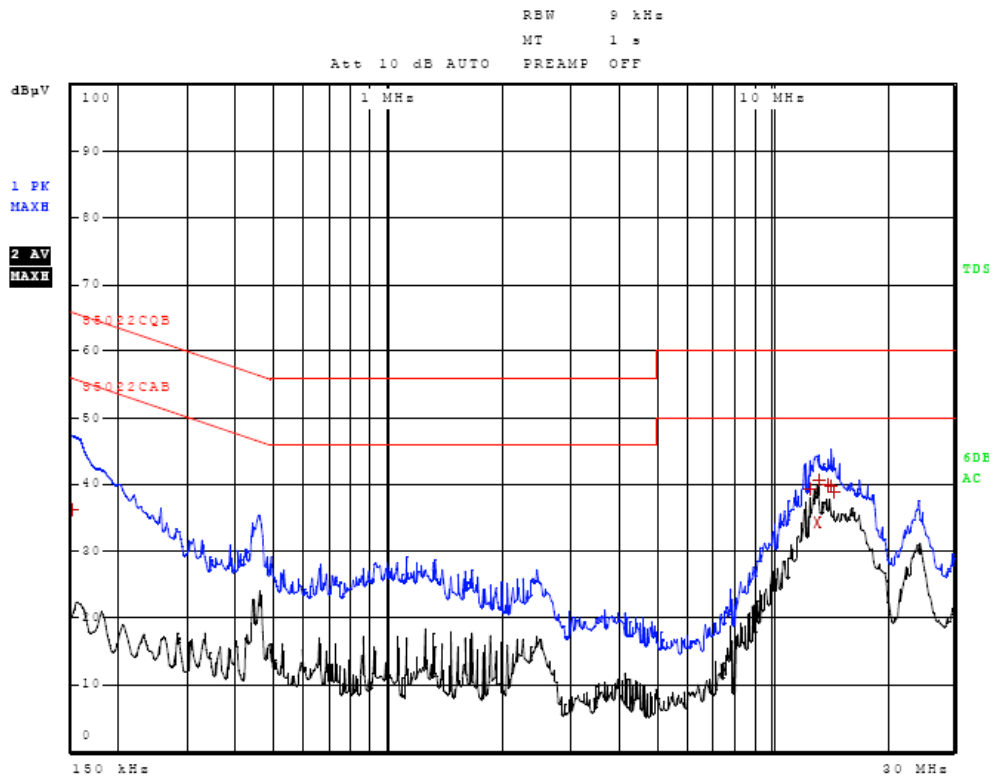
Figure Four AC Line Conducted Emissions Line 2 (configuration 2)
