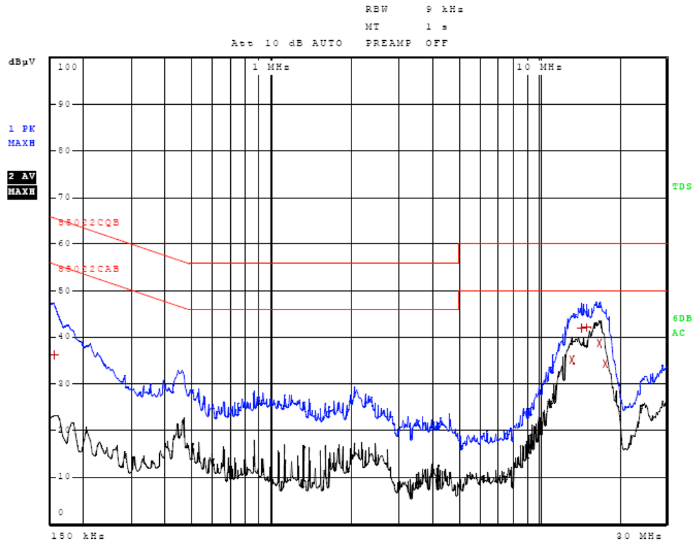
Figure Three AC Line Conducted Emissions Line 1 (configuration 2)
