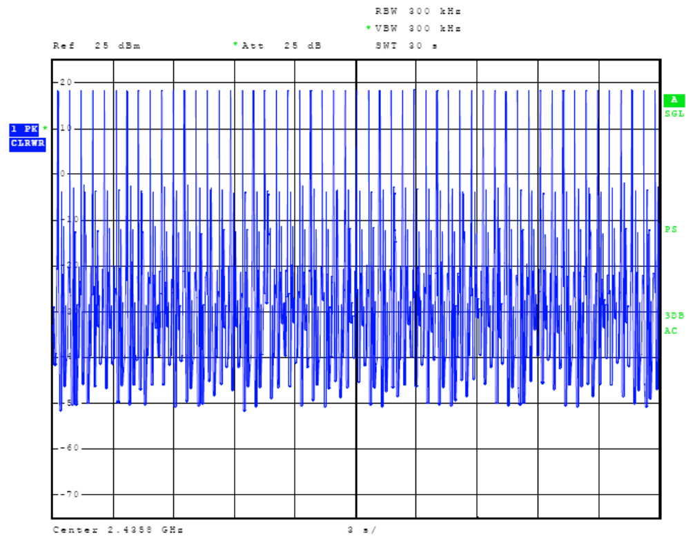
Figure Thirty-five Plot of Channel Occupancy (43 Hop Set)
