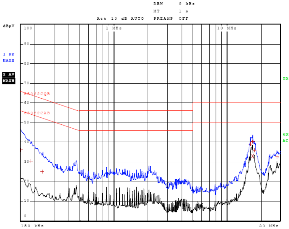
Figure One AC Line Conducted Emissions Line 1 (configuration 1)
