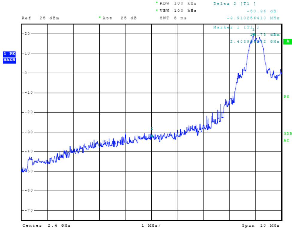
Figure Thirty-eight Plot of Low Band Edge (43 Hop Set)
