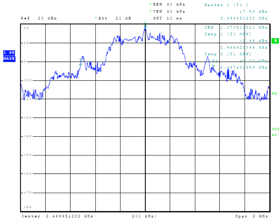
Figure Twenty-nine Plot of 20 dB Occupied Bandwidth (43 Hop Set)
