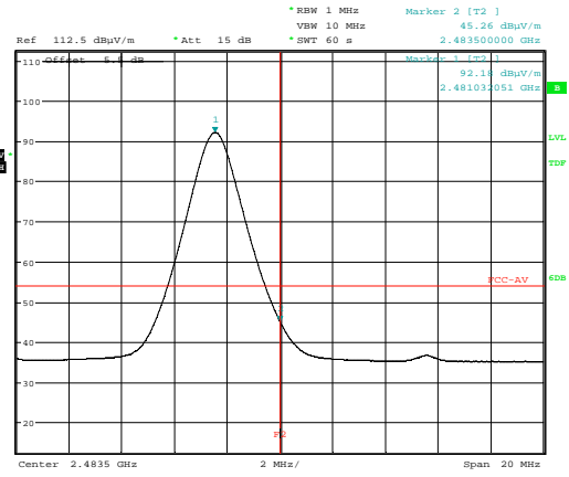
2481 MHz Upper Band Edge Plot - Average
