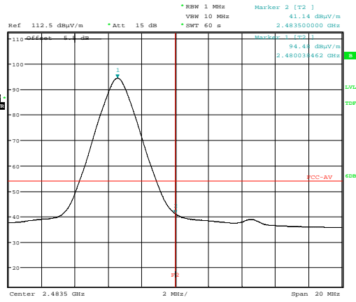
2480 MHz Upper Band Edge Plot - Average
