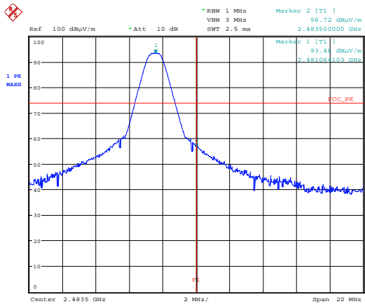
2481 MHz Upper Band Edge Plot – Peak
