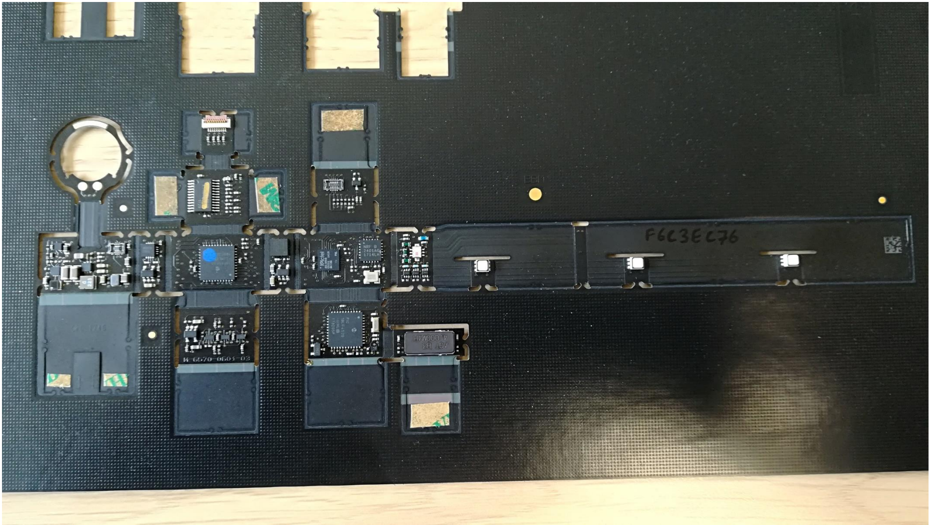
Photo 1. RMP400 Flexi-Rigid PCB Top Side
