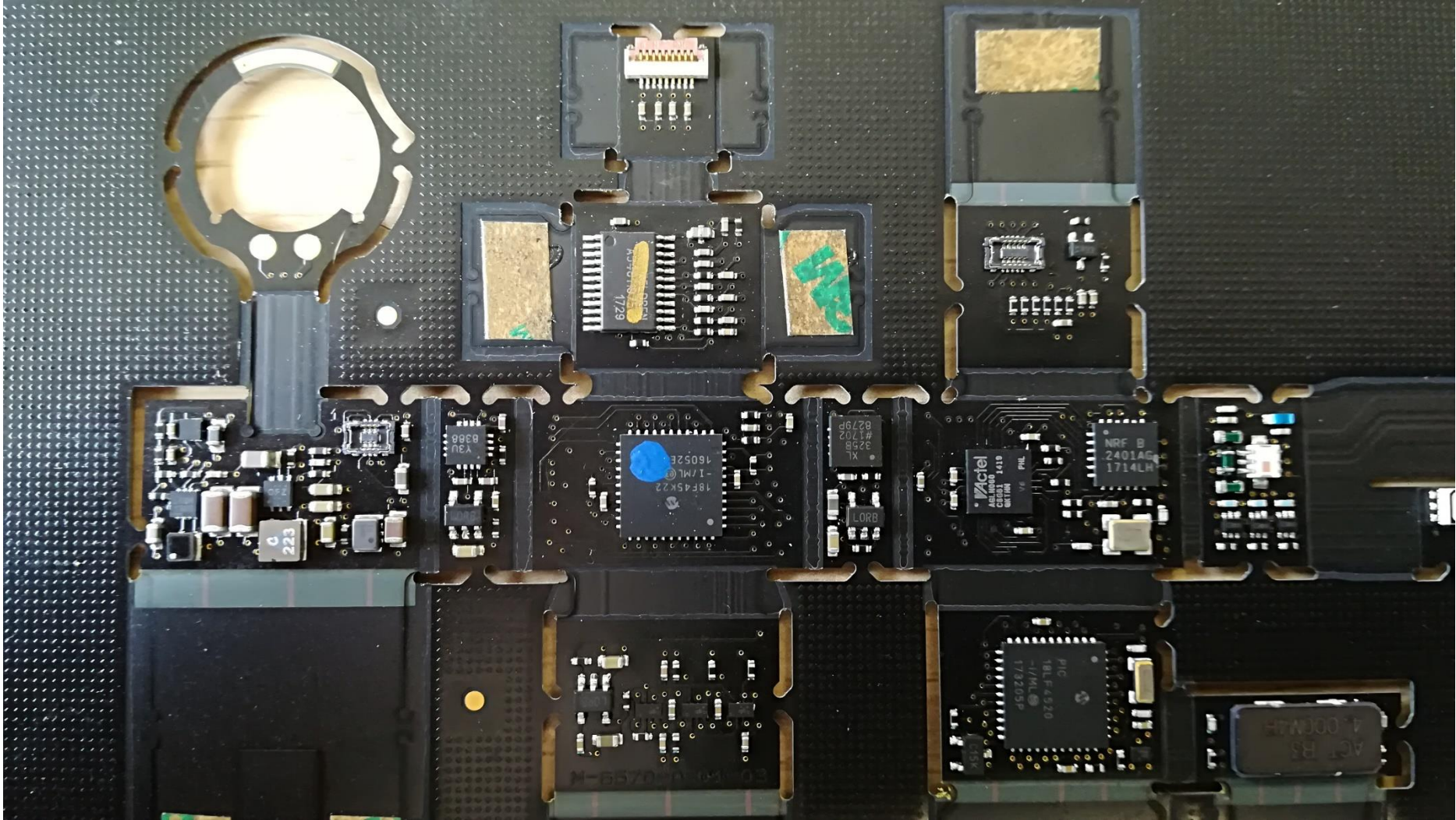
Photo 2. RMP400 Flexi-Rigid PCB Electronics
