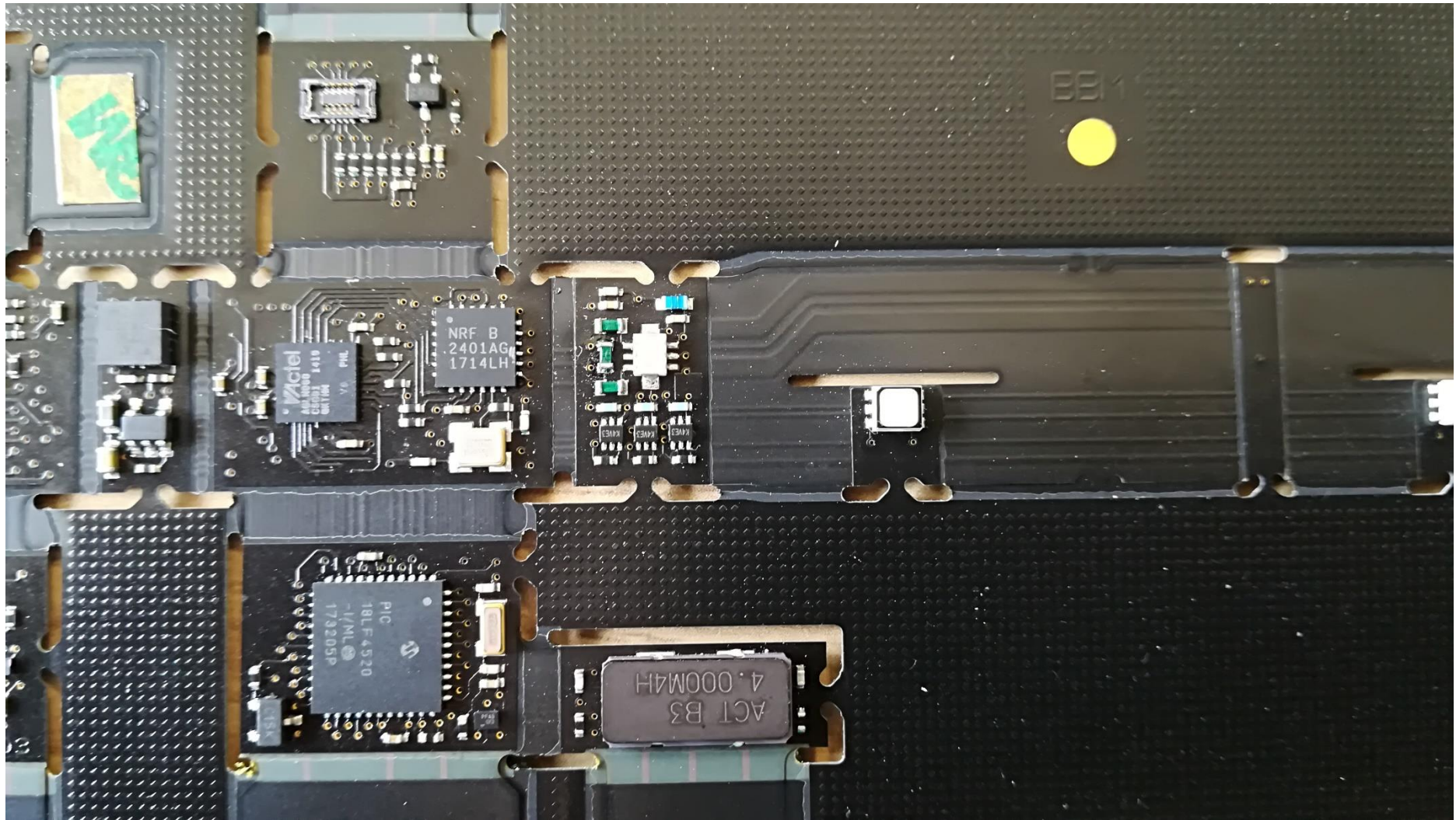
Photo 4. RMP400 Flexi-Rigid PCB Transceiver, matching and transmission line
