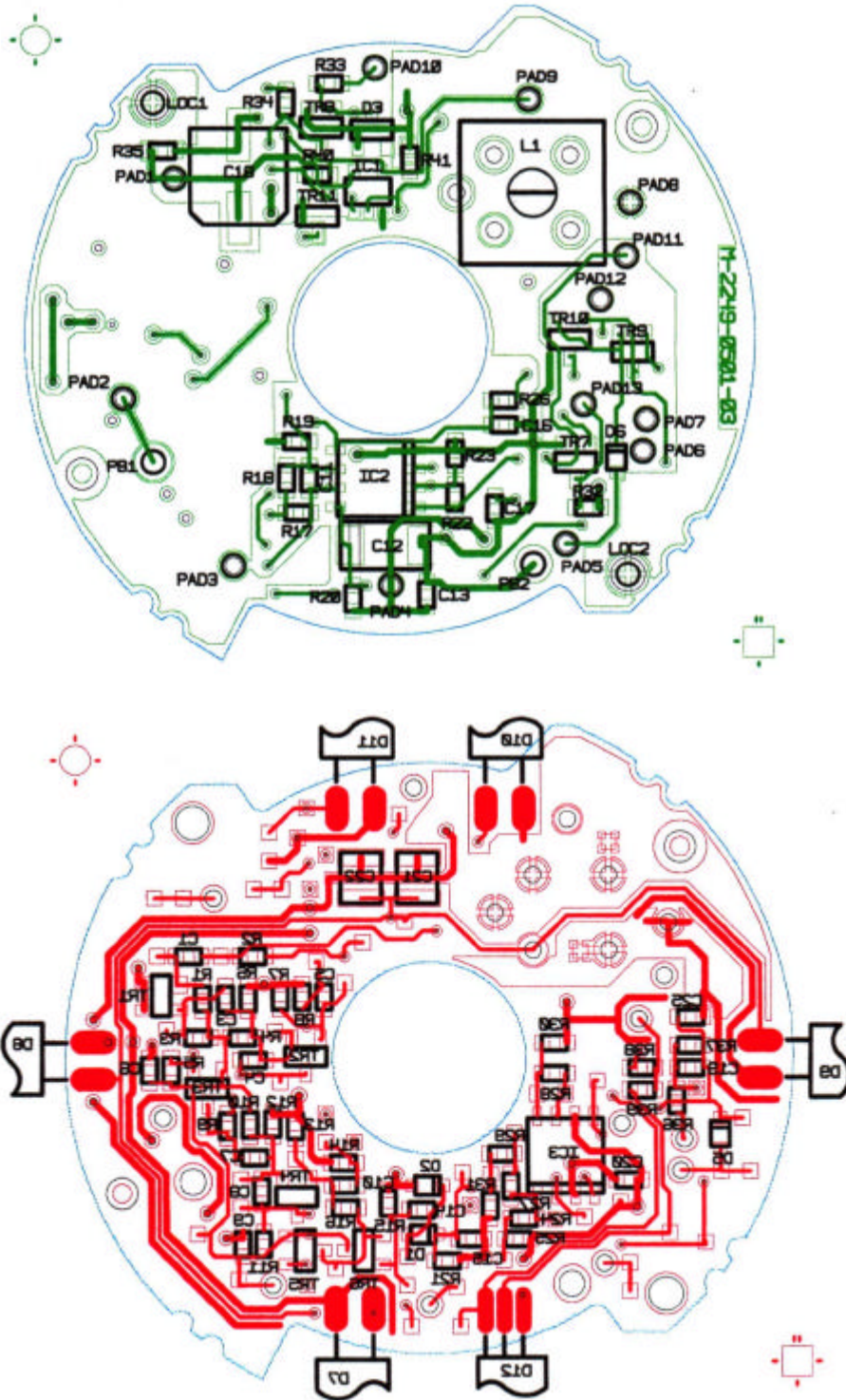
Title: Optic PWB top and bottom
