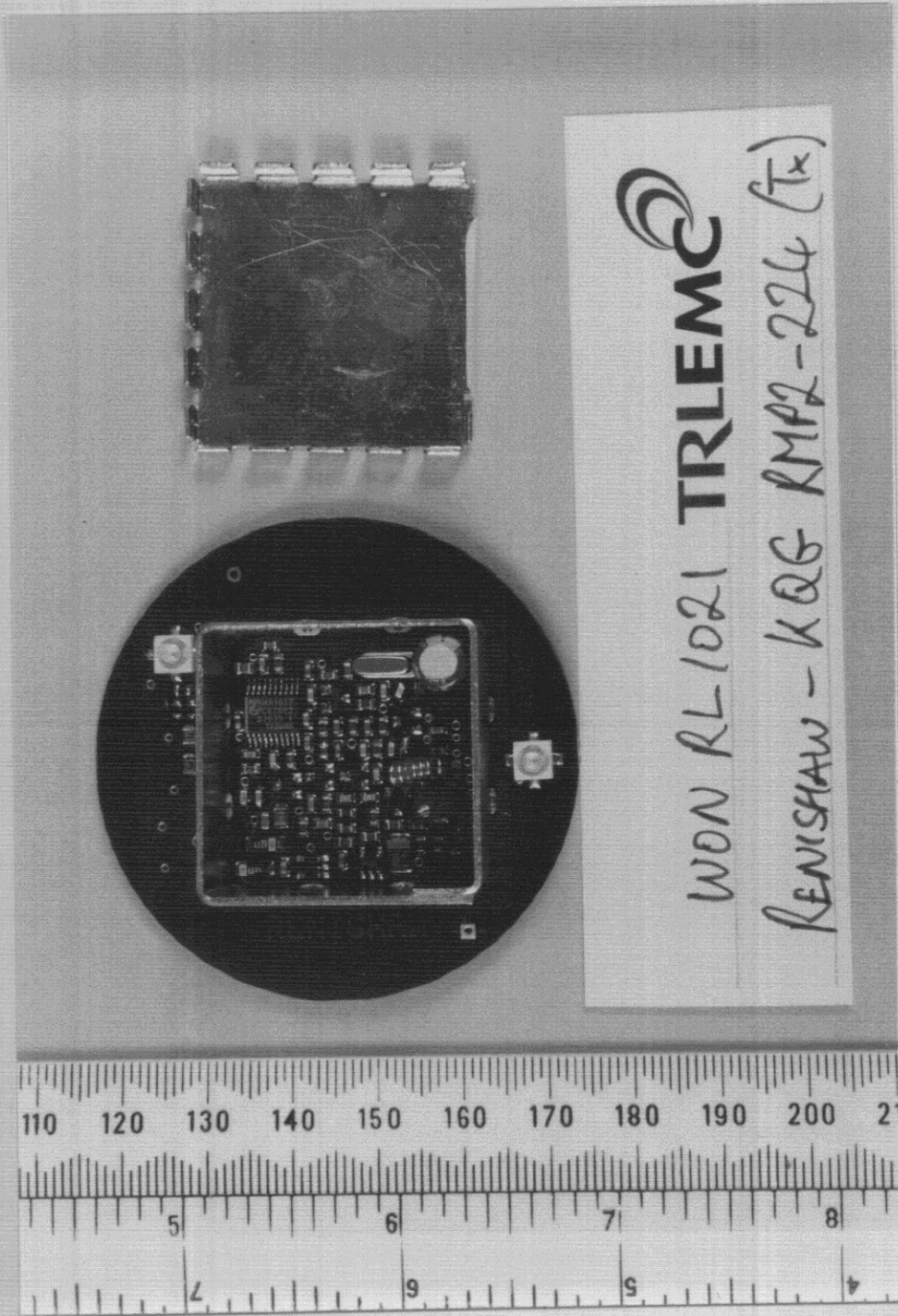
Photograph A4 Title: Tx, rf pcb, top, w/o shield.
