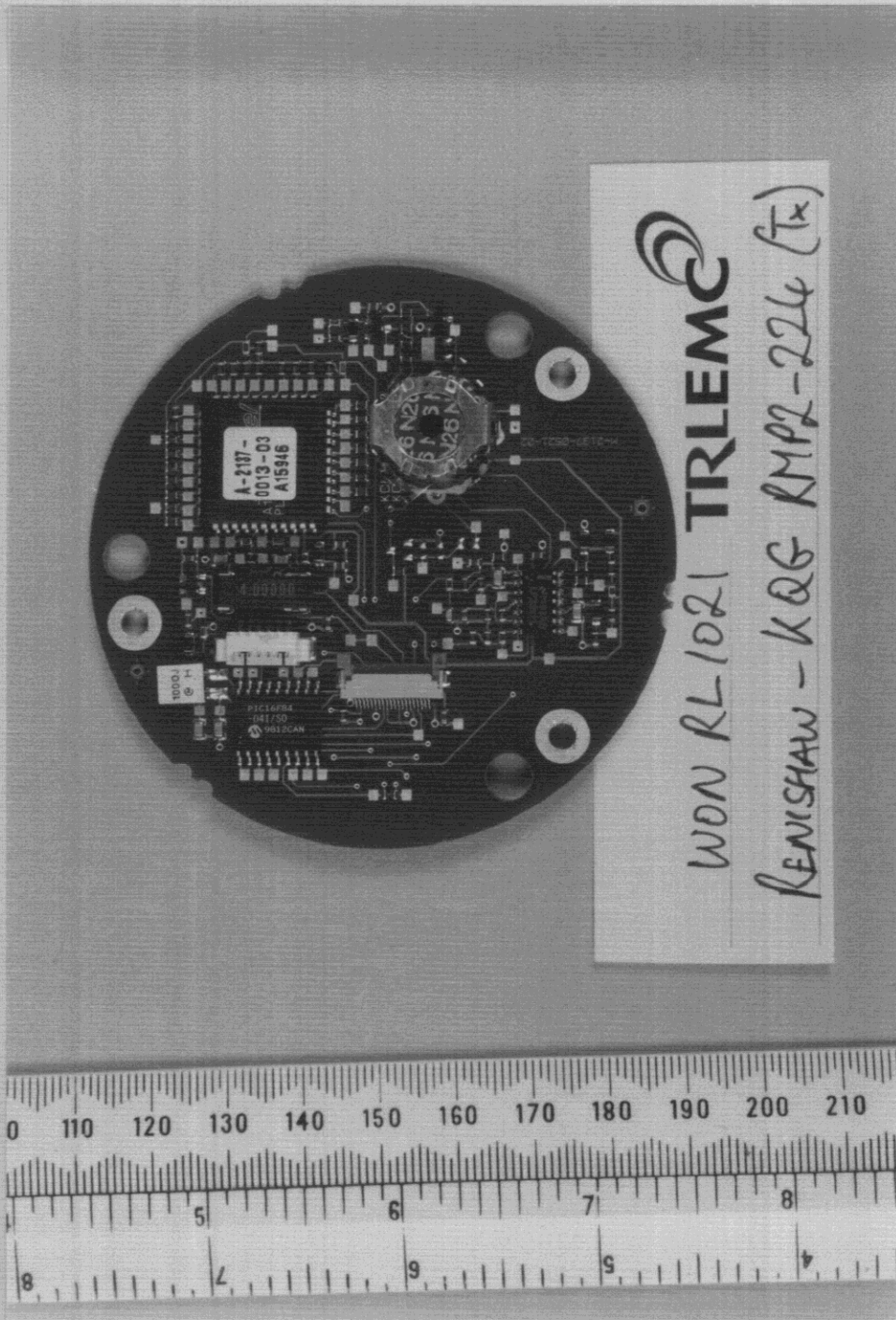
Photograph A6 Title: Logic pcb, top.
