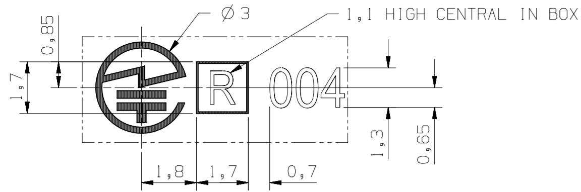
DETAIL M JAPANESE RADIO APPROVAL LOGO (SCALE 8:1)
