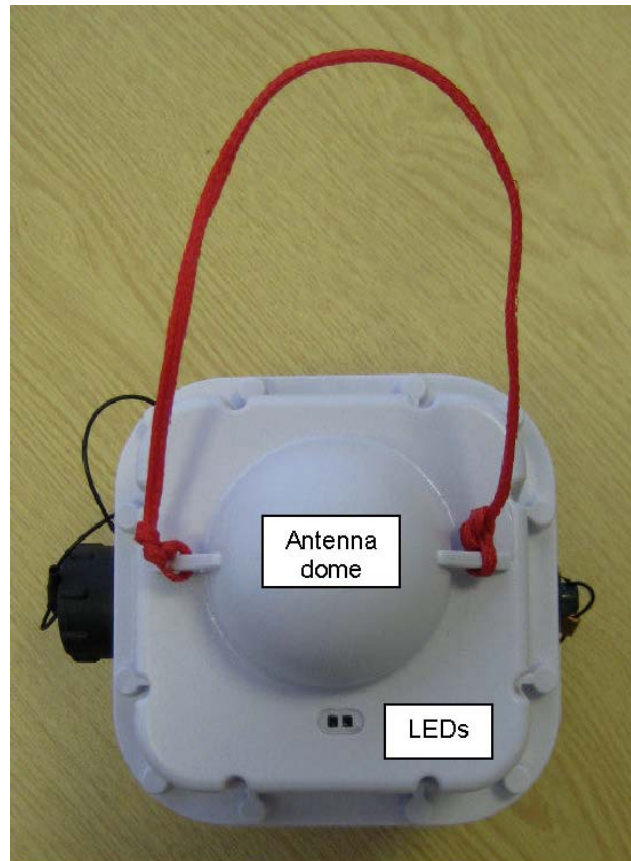
Figure 18 : Vibtech Unite unit (top)
