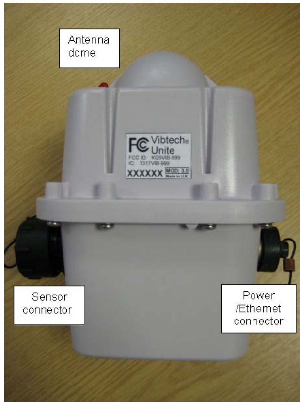
Figure 14 : Vibtech Unite unit (front)
