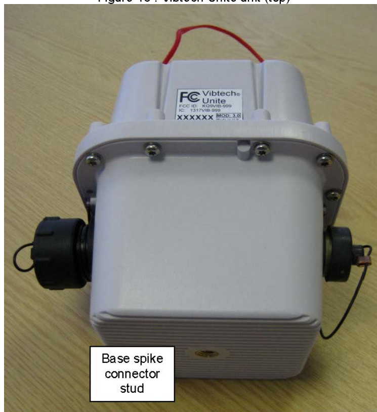
Figure 19 : Vibtech Unite unit (base)
