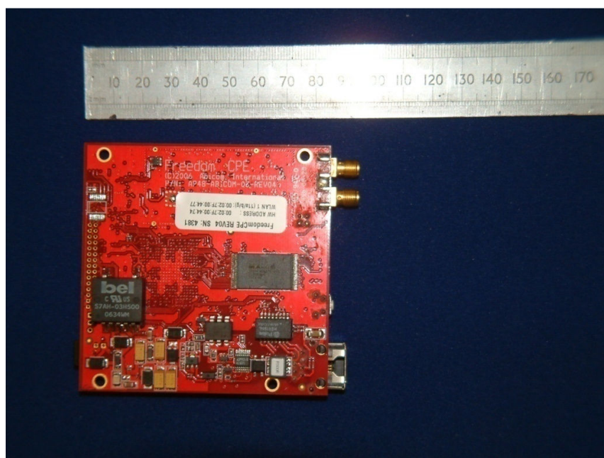
CPE Module S/N 4381 (Bottom Face)
