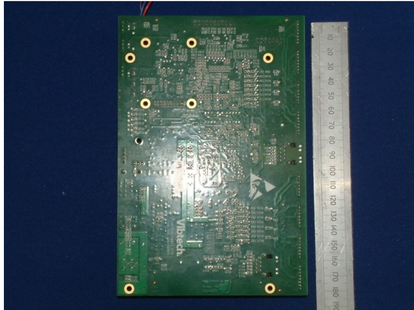
CAN II Motherboard (Bottom Face)
