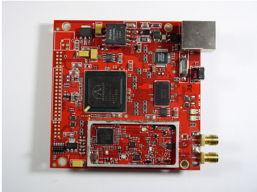
Top Face of CPE Module – Shielding Removed
