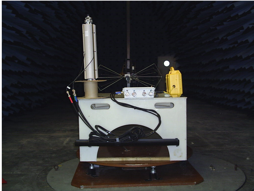
3m Open Area Test Site
