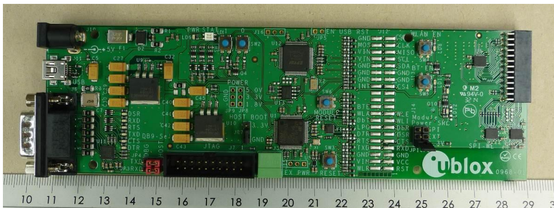
145298_27.jpg: Adaptor Board – Top View
