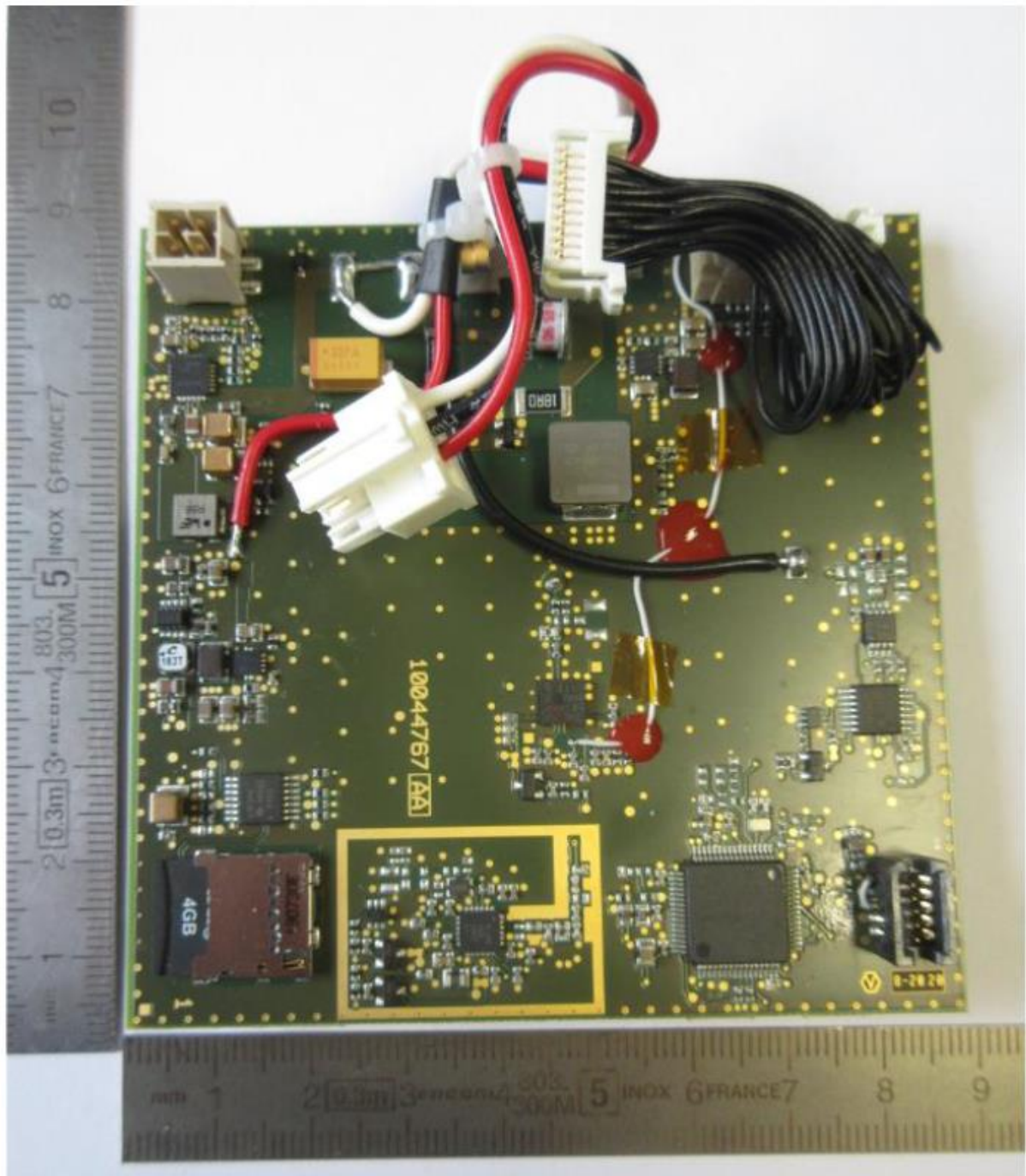
DFU board
