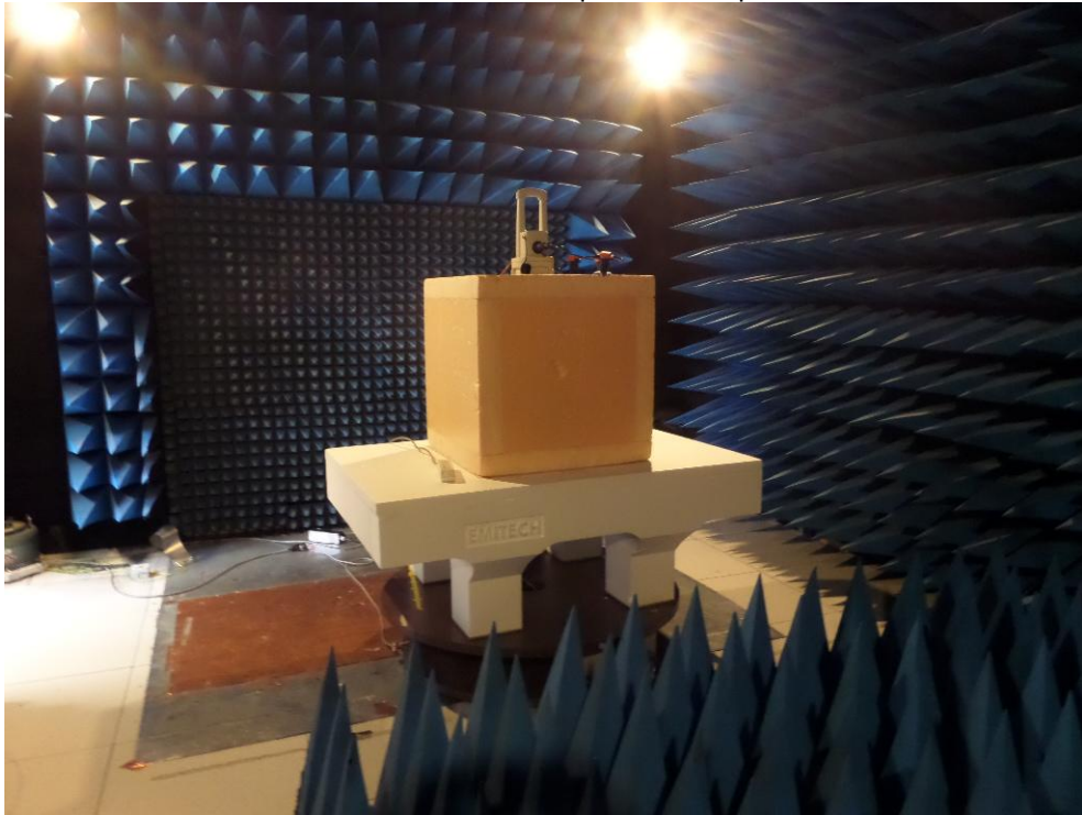
Anechoic chamber product setup
