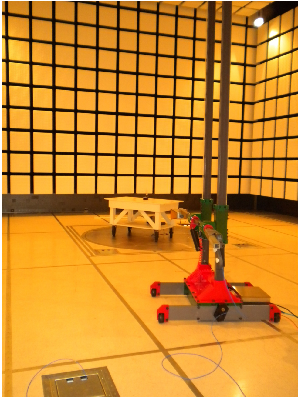
Setup Photo for Radiated Spurious Emissions Testing:
