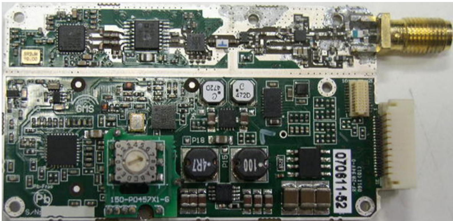
Figure 6 Component Side View main board Assy, VMT 700-A0985X3A-G
