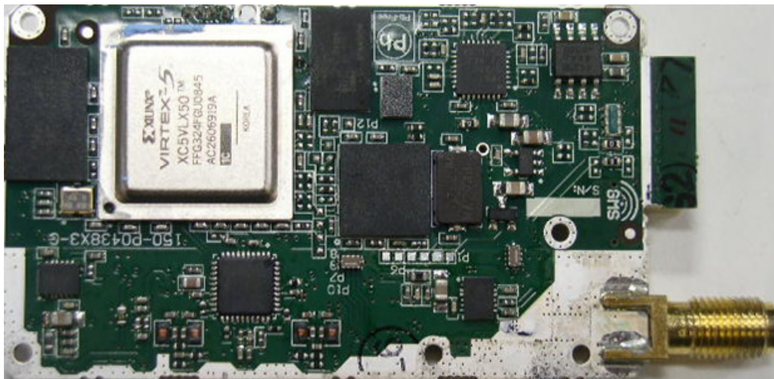
Figure 5 Soldered Side View main board Assy, VMT 700-A0985X3A-G
