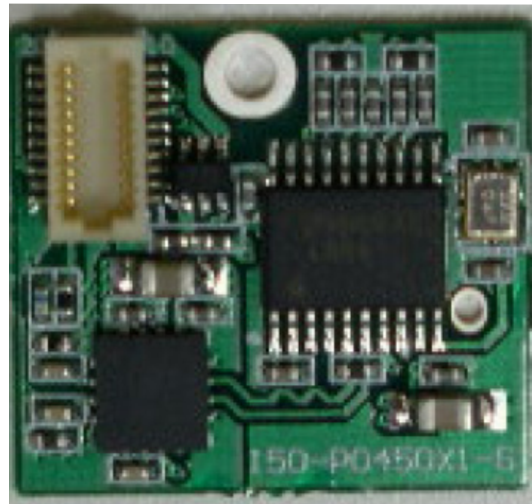
Figure 2 Component Side View SD-SDI interface board 700-A1009X1-G
