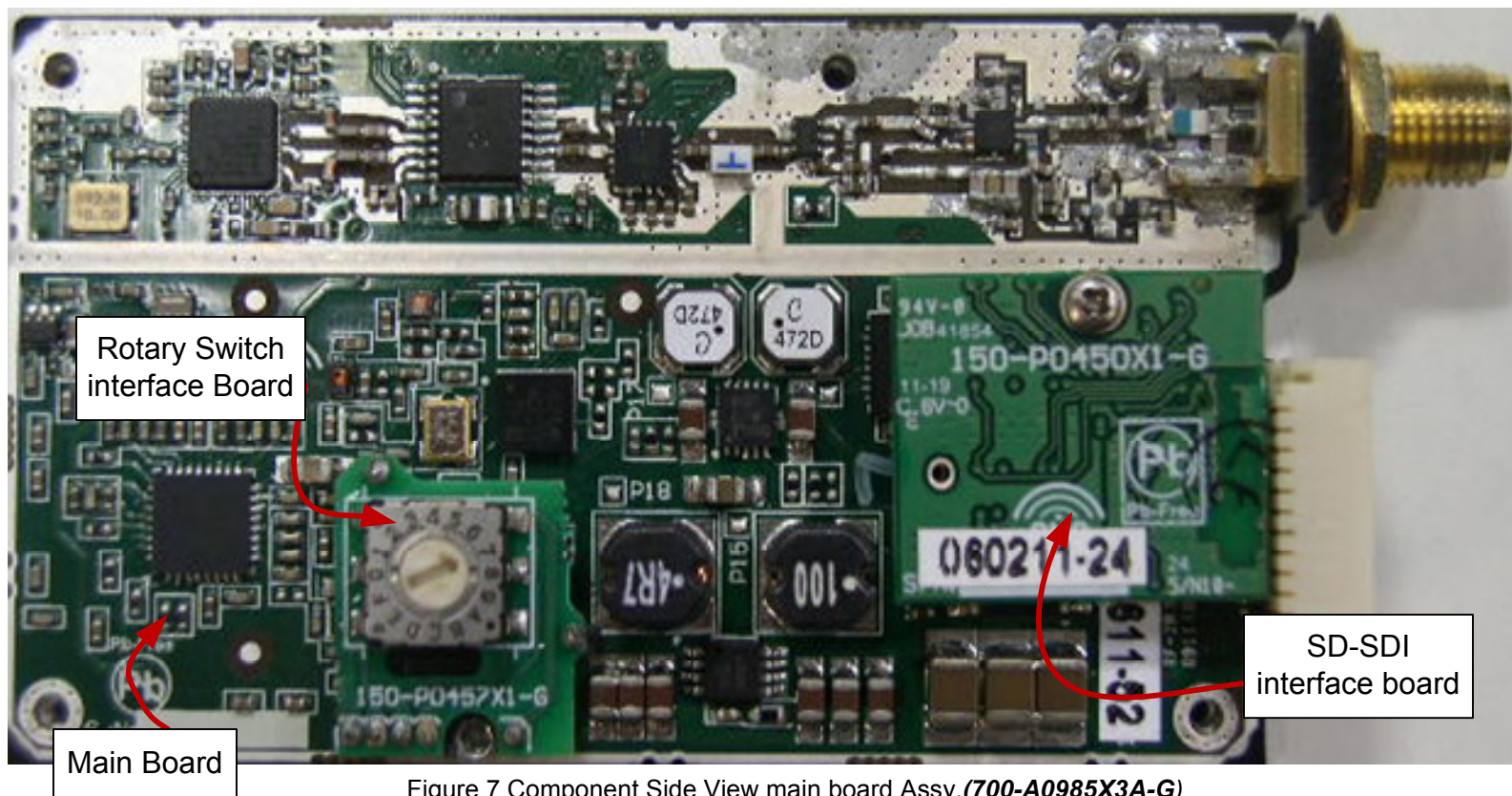
Figure 7 Component Side View main board Assy, (700-A0985X3A-G) with SD-SDI interface board (700-A1009X1-G) and Rotary Switch interface board (700-A1057-G)
