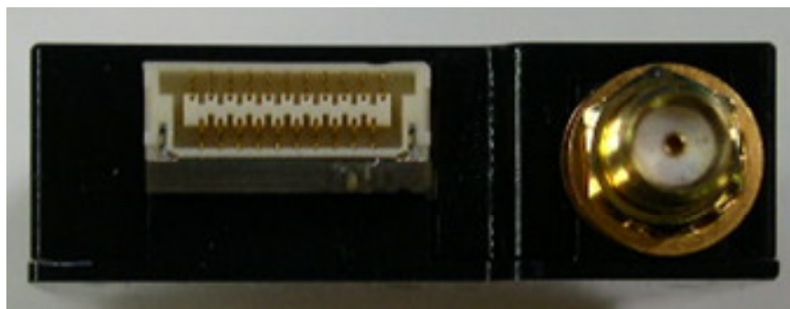
Figure 5 Front Side View with RF SMA connector & I/O connector
