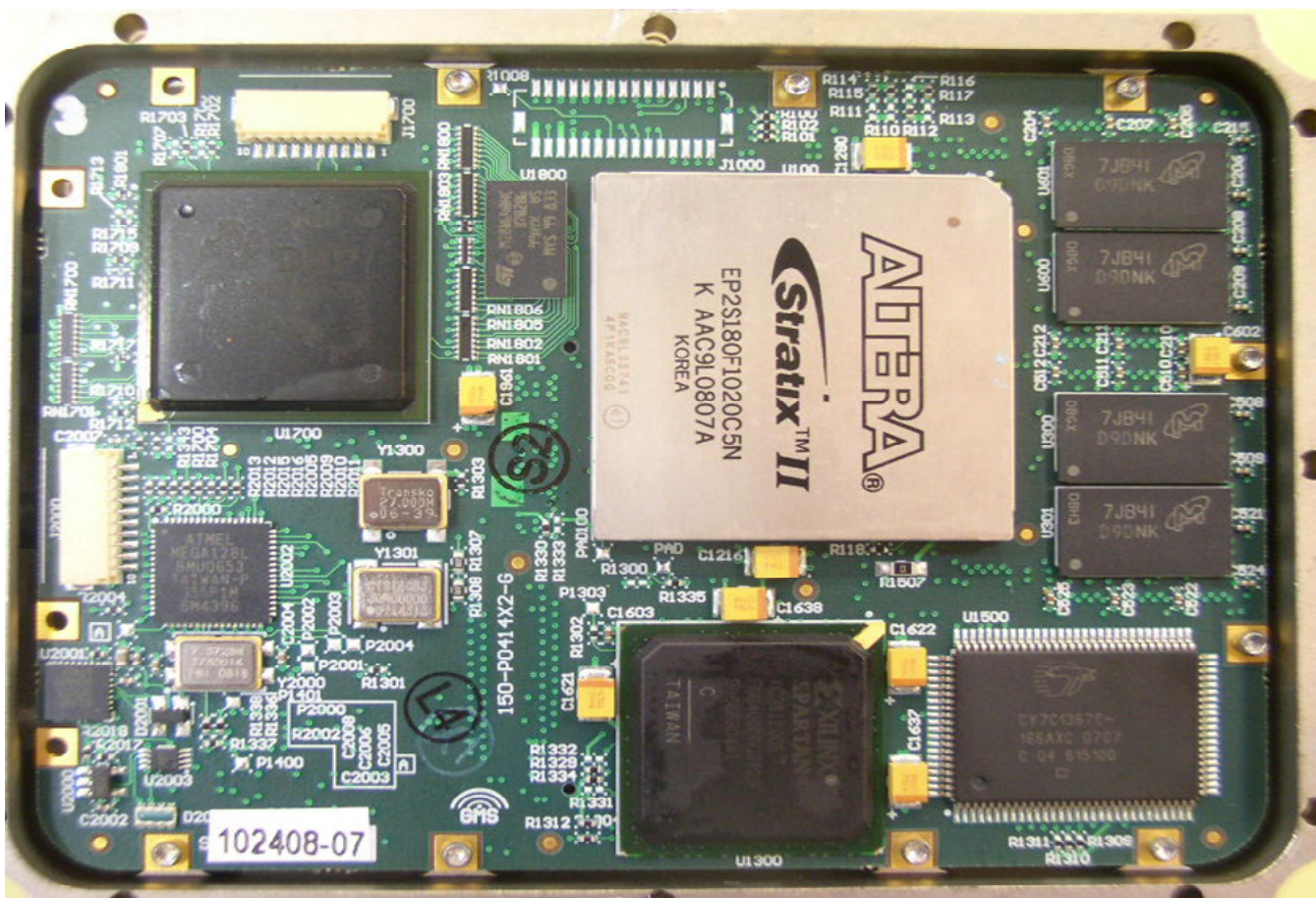
Figure 2_Internal_AVC encoder_component_side_700-A0864
