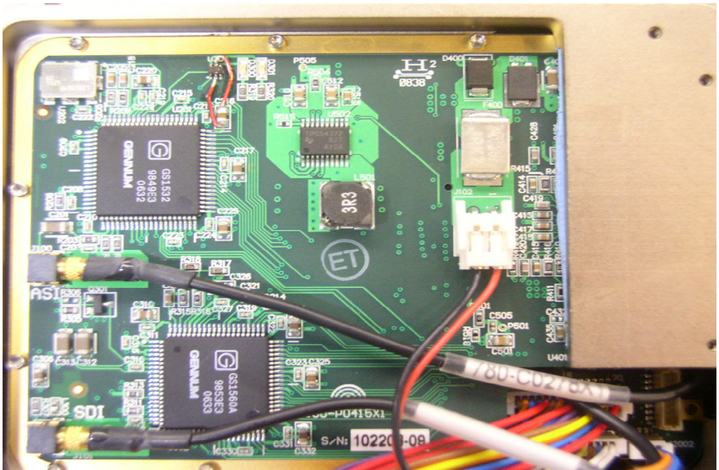
Figure 3_ internal_AVC_PowerSupply_component_side_700-A0865
