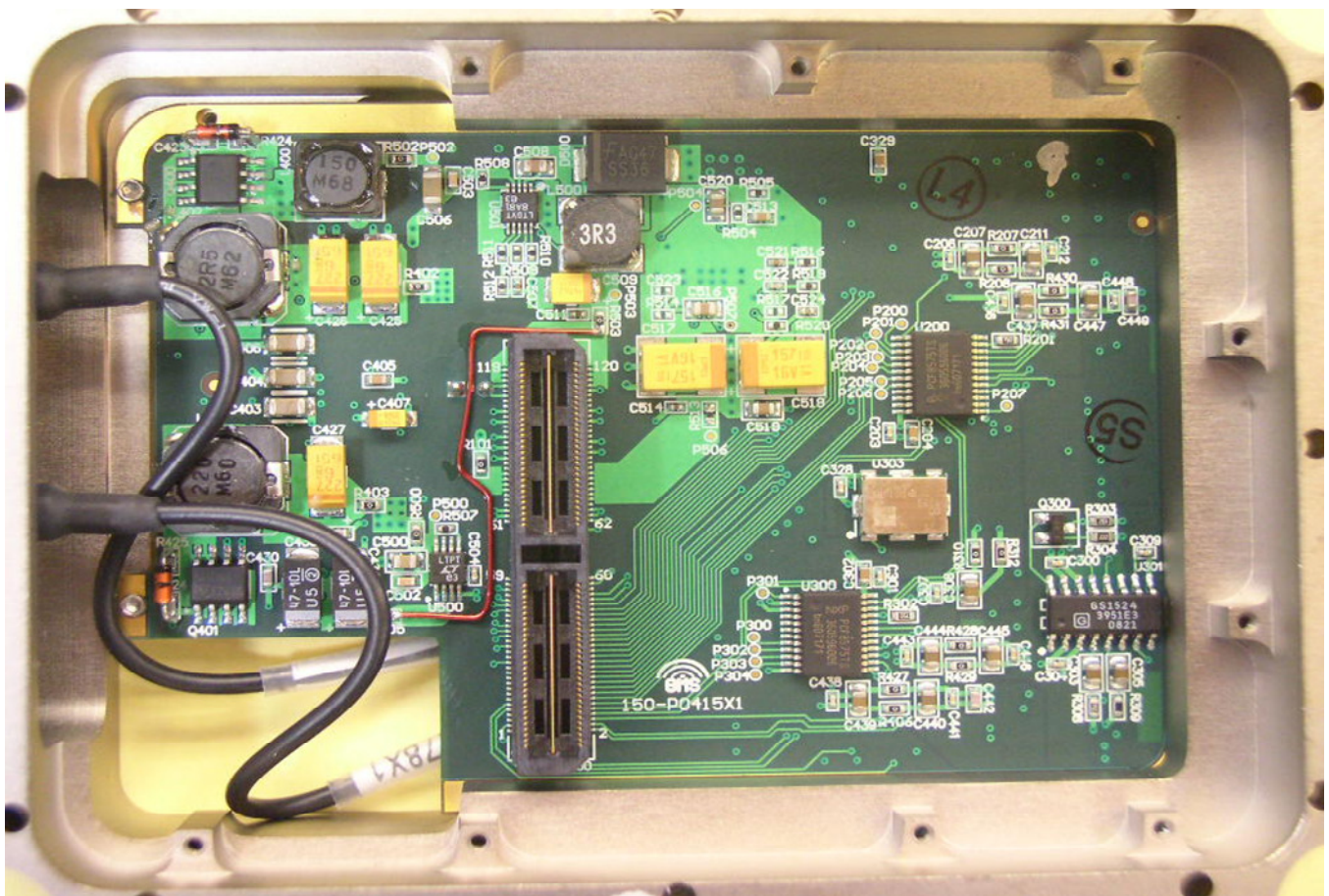
Figure 4_ internal_AVC_PowerSupply_solder_side_700-A0865
