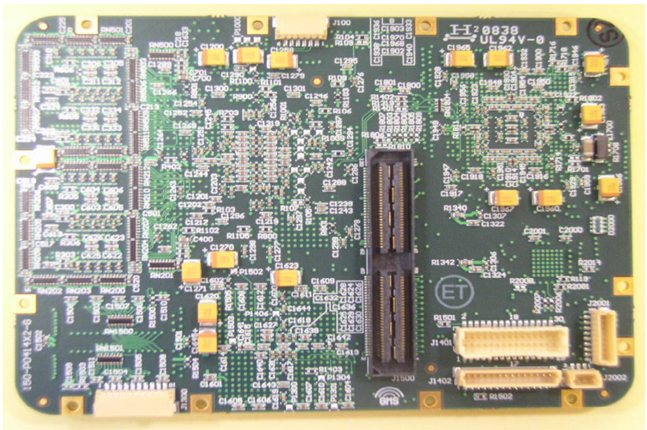
Figure 1_internal_AVC_encoder_solder_side_700-A0864
