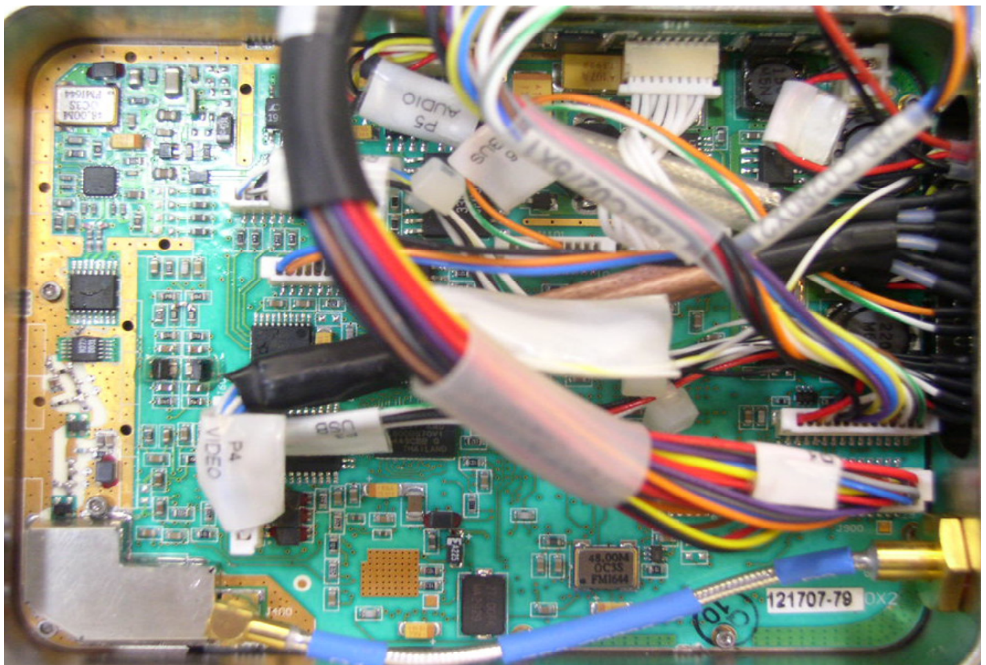
Figure 6_ internal_MDT3_component_side_700-A0750
