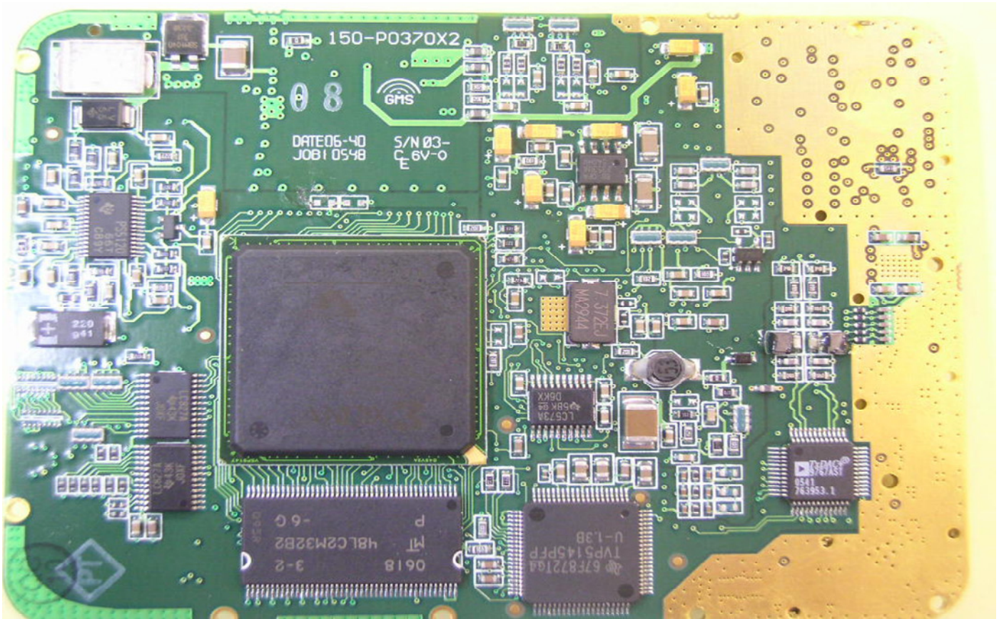
Figure 5_ internal_MDT3_solder_side_700-A0750
