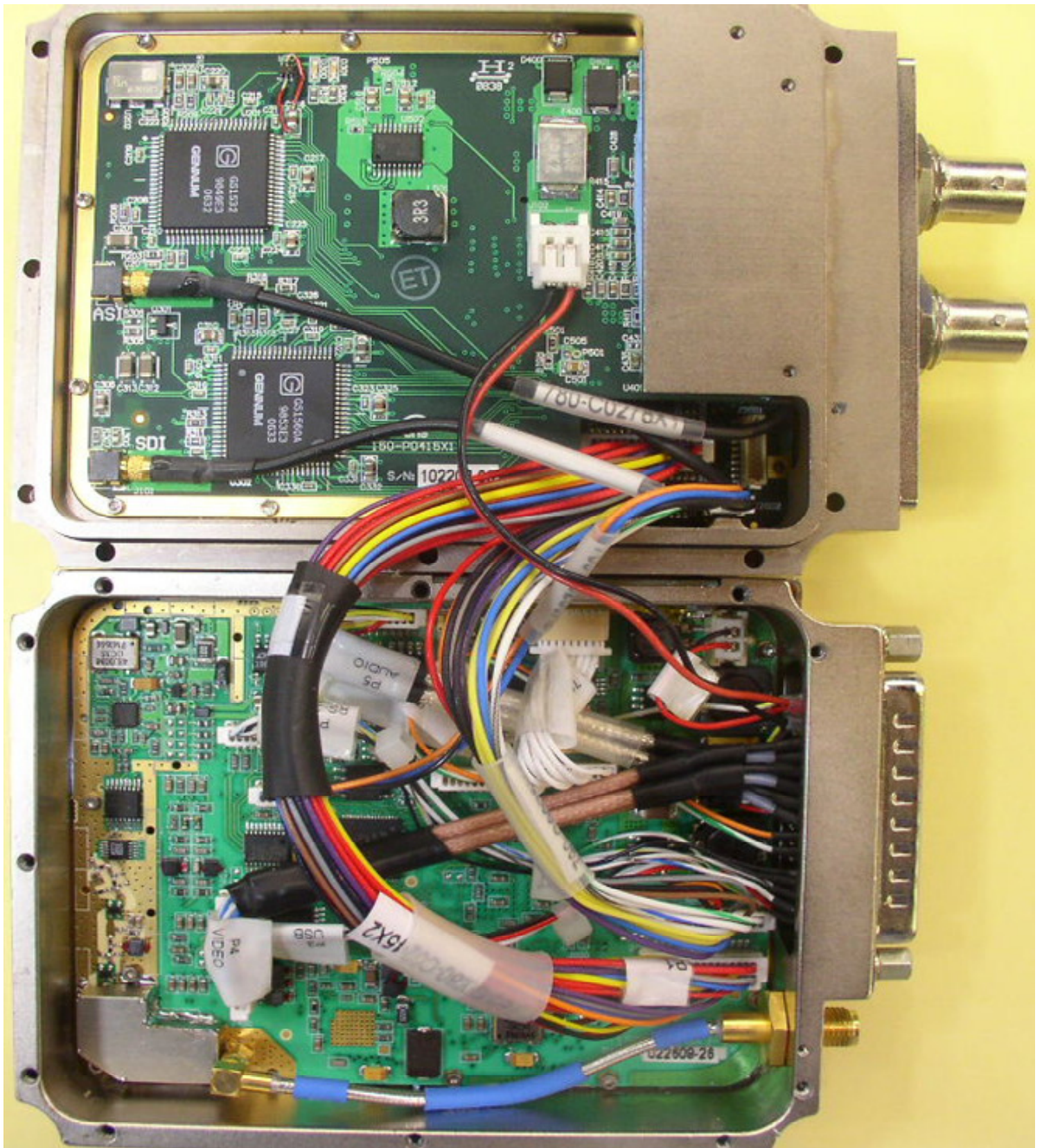
Figure 7_ internal_MDT3_with AVC encoder module
