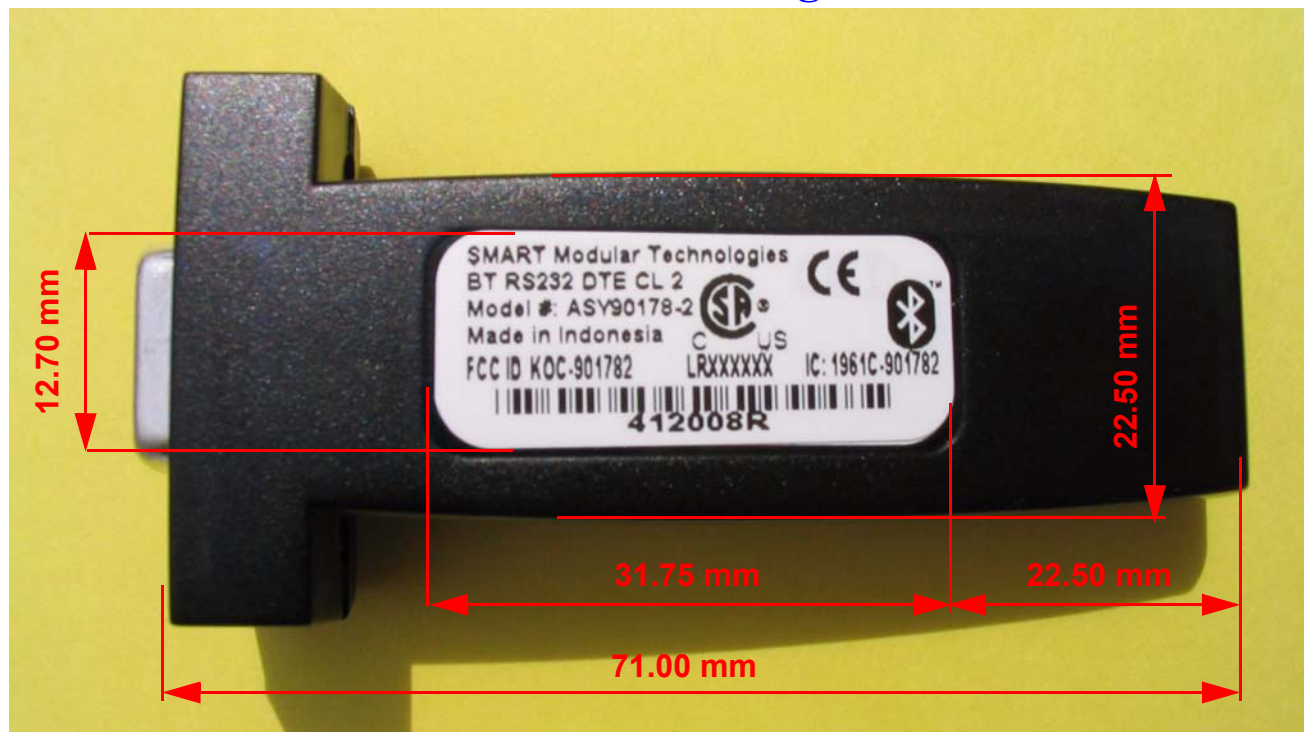
Bottom View - Bluetooth RS232 DTE Class 2, Model ASY90178-2
