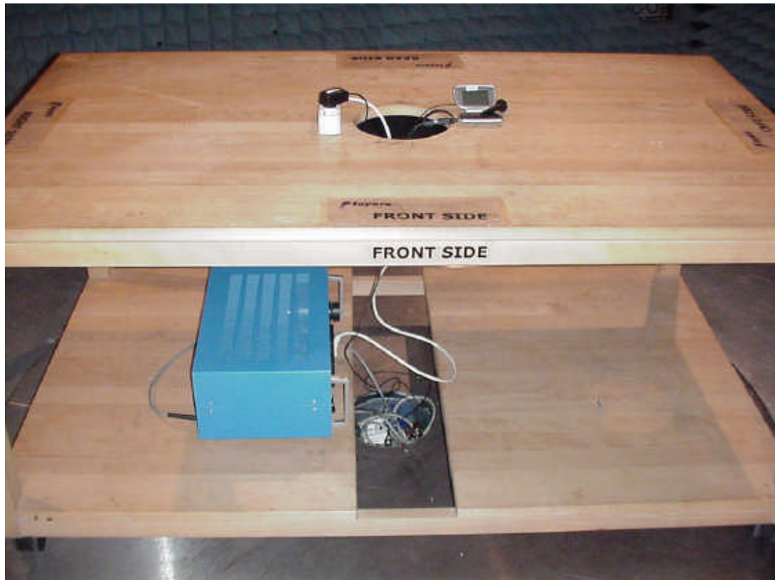
Photo1: EUT A (neochat) with PI charger
