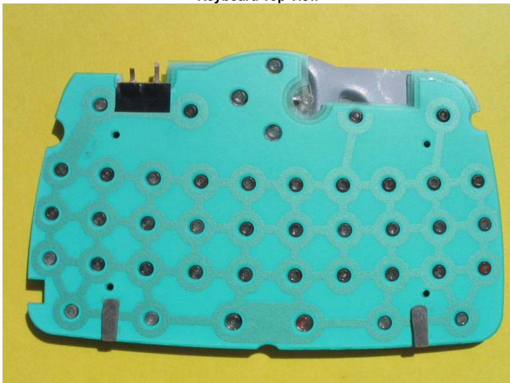
Keyboard Bottom View
