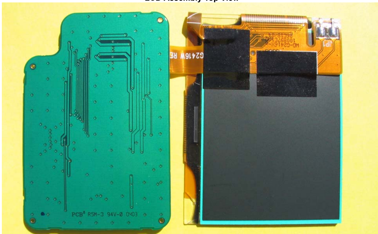
LCD Assembly Bottom View
