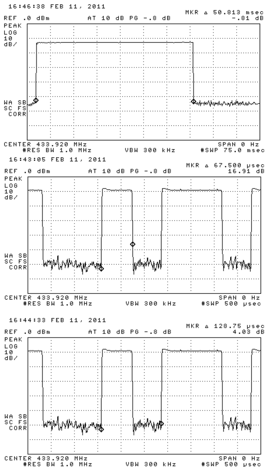
Figure 6.1(b). Manchester encoded ASK Frame characteristics. (top) frame length, (center) Manchester packet length , (bottom) Manchester packet period.
