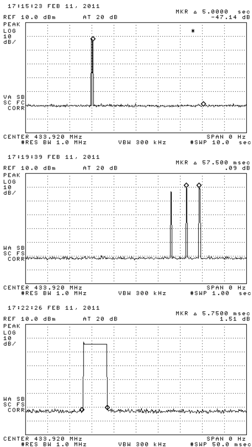
Figure 6.1(d). Manual LF Activated FSK Transmission. (top) 5 second turn-off after door-handle release, (center) LF activated Transmission (max of two frames per 100 ms window), (bottom) FSK frame length.
