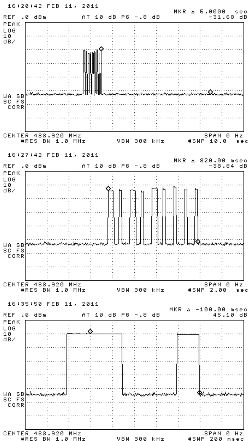
Figure 6.1(a). Manual Button Press Transmission characteristics. (top) 5 second turn-off after release, (center) Transmission from single button press (a minimum length press would show only 3 repeated pairs of frames (ASK frame then FSK frame, ASK then FSK, ASK then FSK) , (bottom) worst-case 100 ms window.
