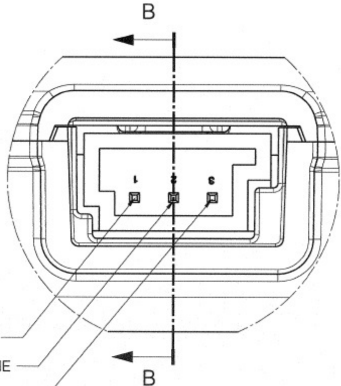
Detail A Scale: 5:1 3WAY CONNECTOR FACE VIEW
