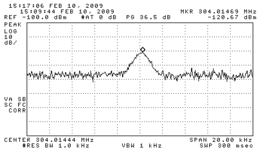
Figure 6.3. Relative receiver emission(s). LO was not detectable.
