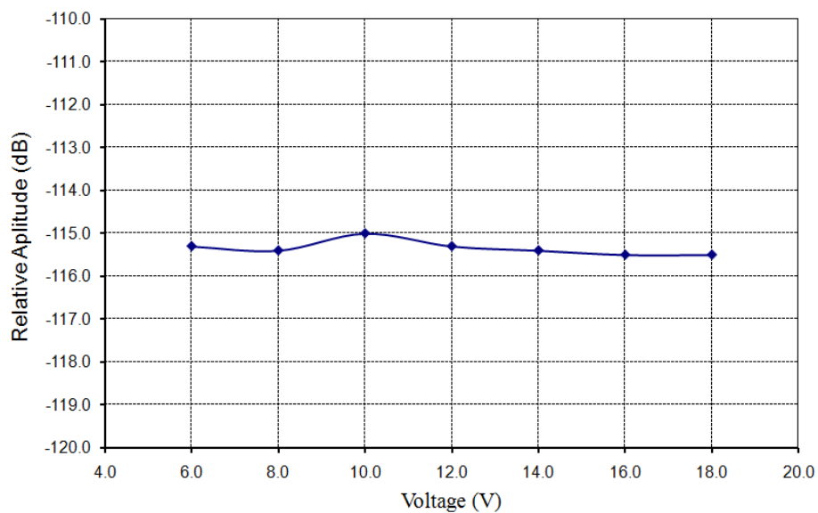
Figure 6.4. Relative emission vs. supply voltage.
