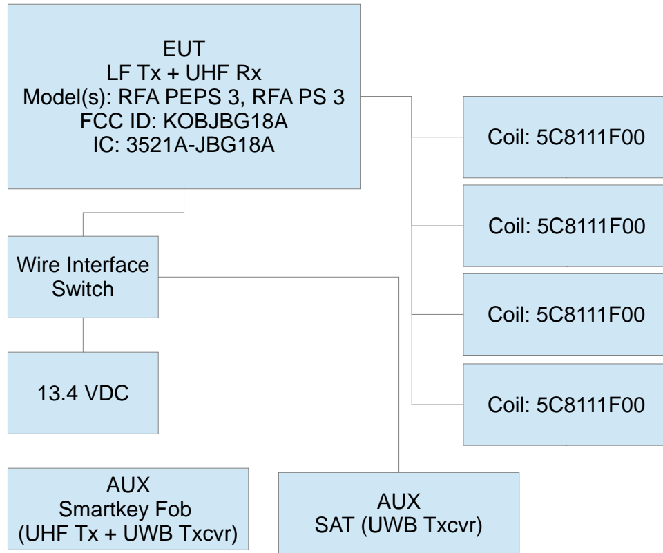
Figure 2: EUT Test Configuration Diagram.
