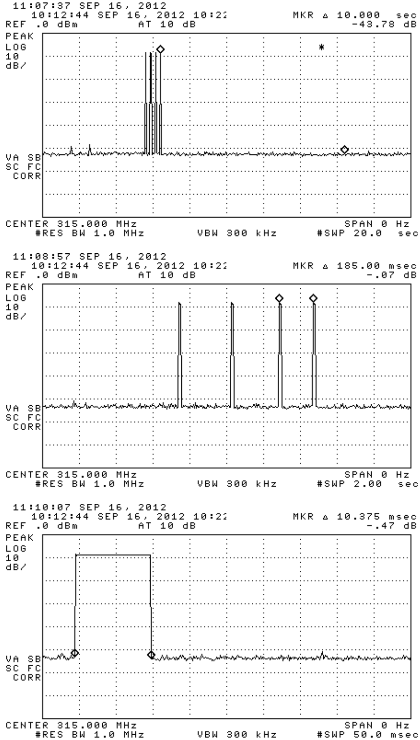
Figure 6.1. Transmission modulation characteristics. (top) complete transmission, (center) expanded transmission, (bottom) single FSK frame.
