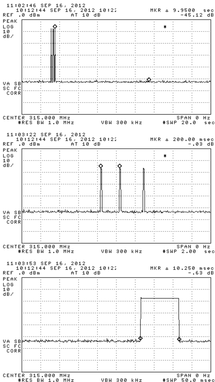
Figure 6.1. Transmission modulation characteristics. (top) complete transmission, (center) expanded transmission, (bottom) expanded frame.
