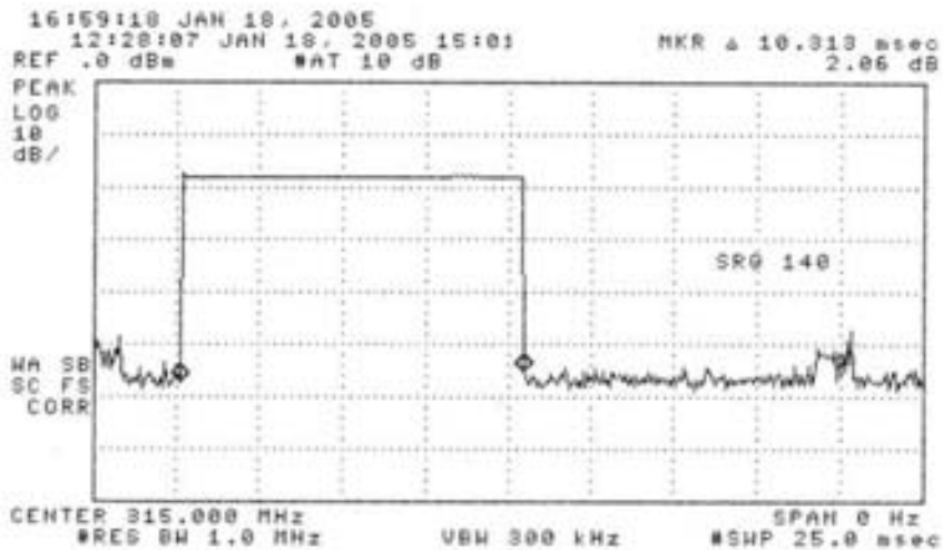
Figure 6.1. Transmissions modulation characteristics: (top) low line transmission, (center) high line, (bottom) expanded word (same for high and low line).
