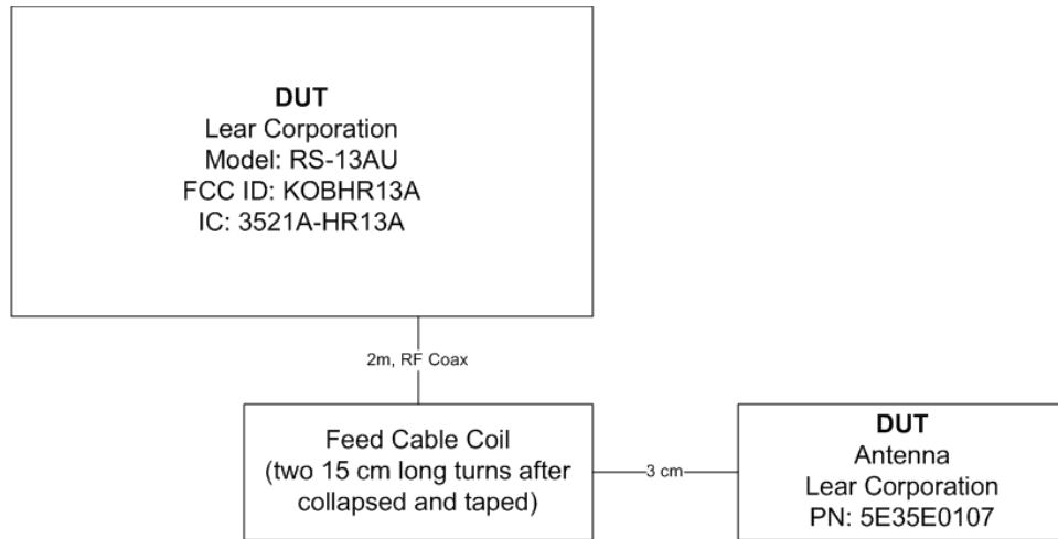
Figure 3.1 Block Diagram
