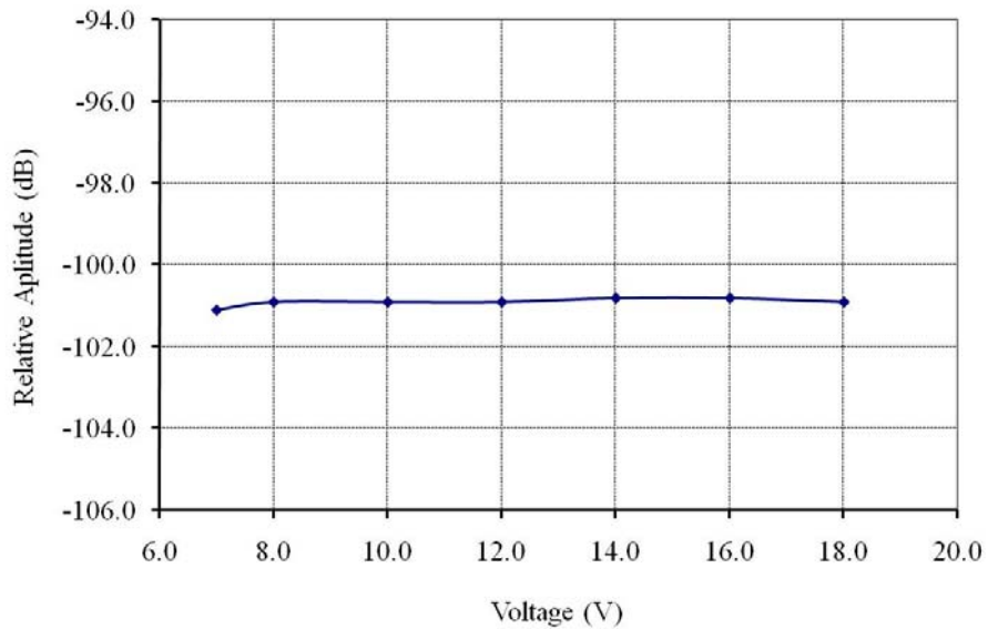
Figure 6.2. Relative emission vs. supply voltage.
