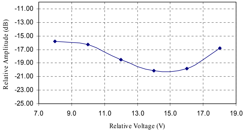
Figure 6.4. Relative emission at 135 kHz vs. supply voltage.
