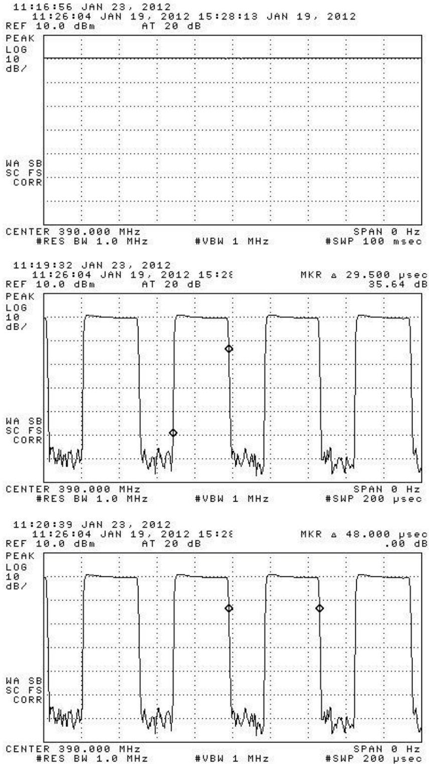
Figure 6.1(i). Transmission modulation characteristics 390 MHz. (top) maximum on time transmission, (center) Manchester bit width, (bottom) Manchester bit period.
