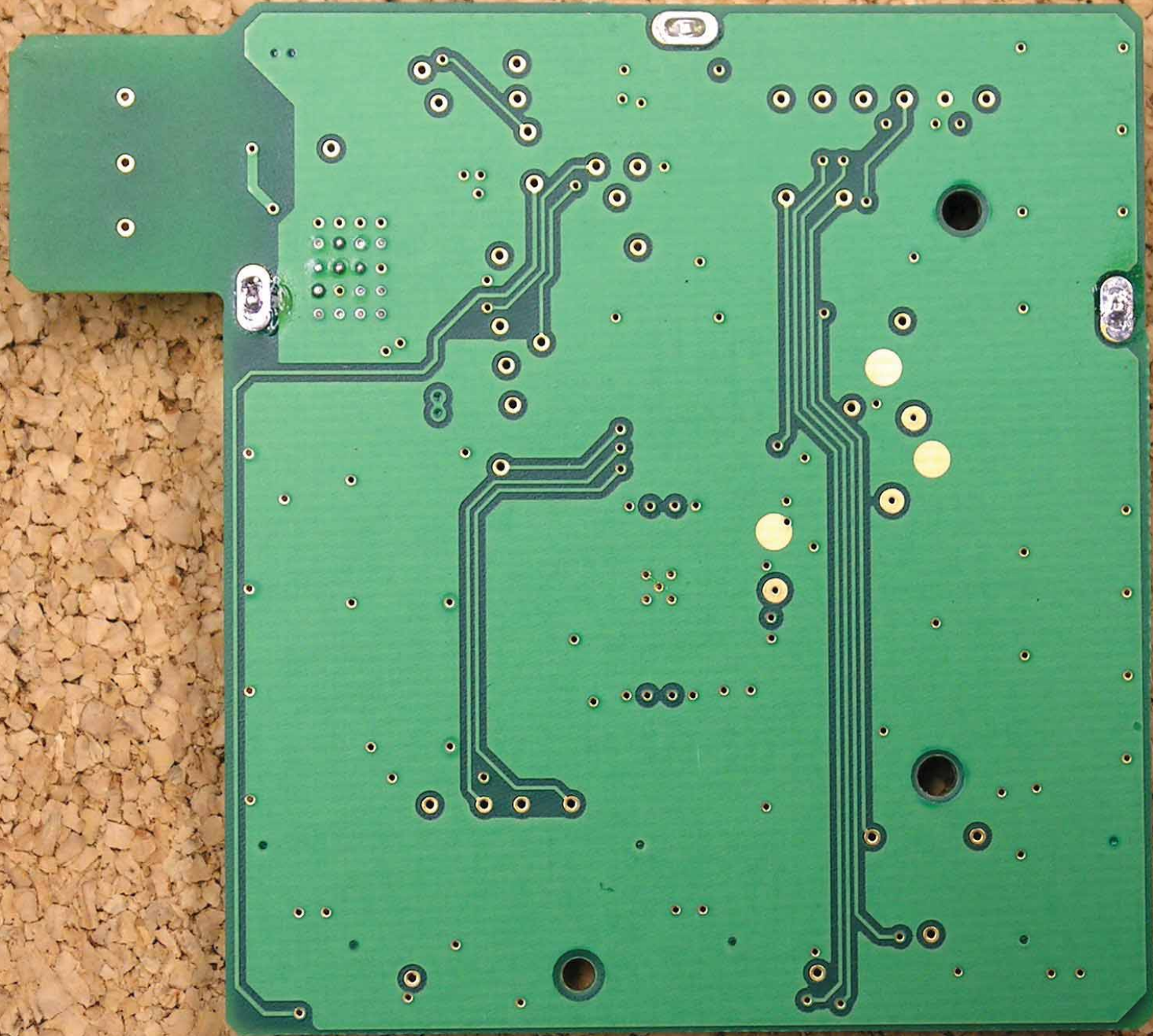
PCB (bottom)
