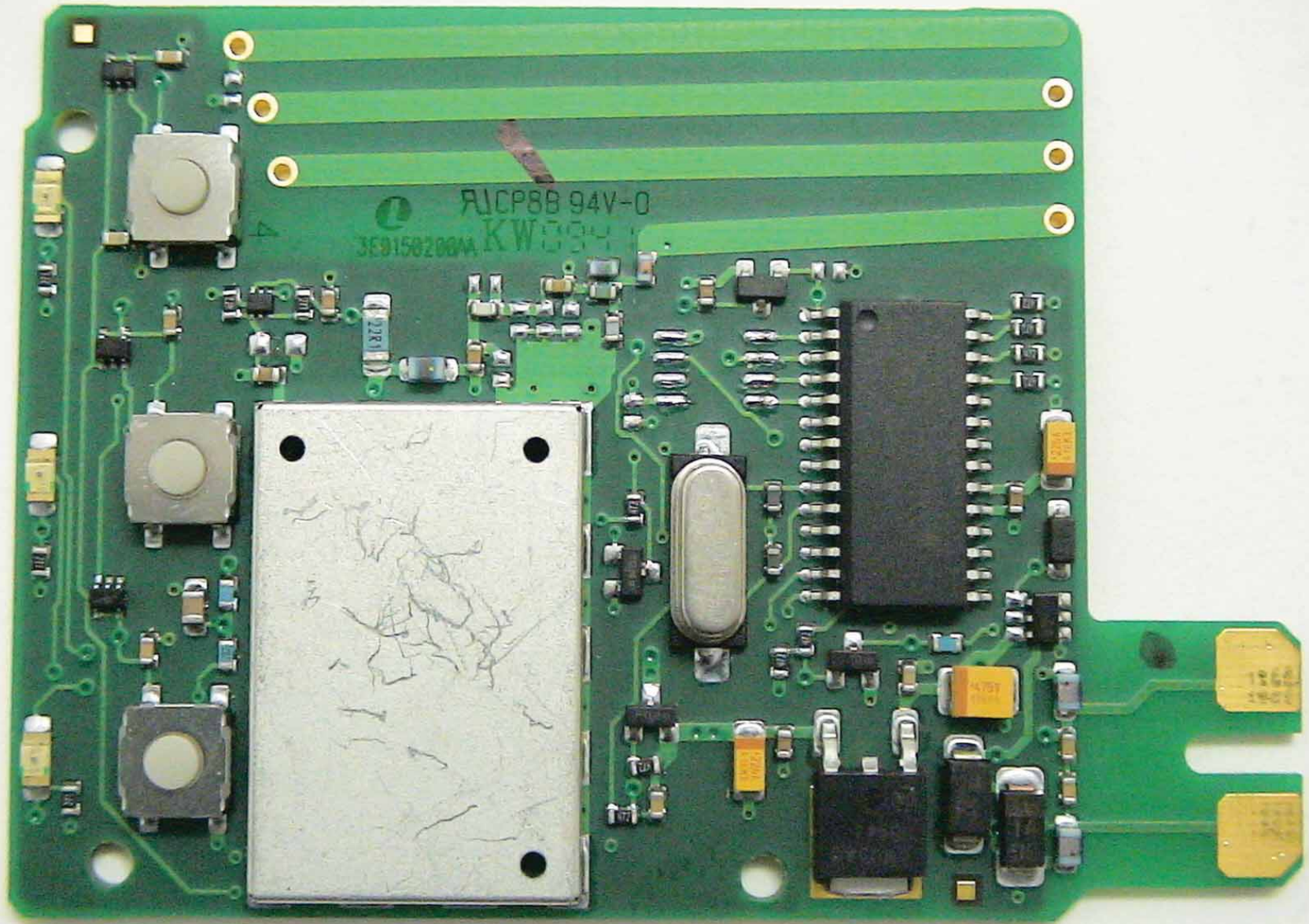
PCB (top)
