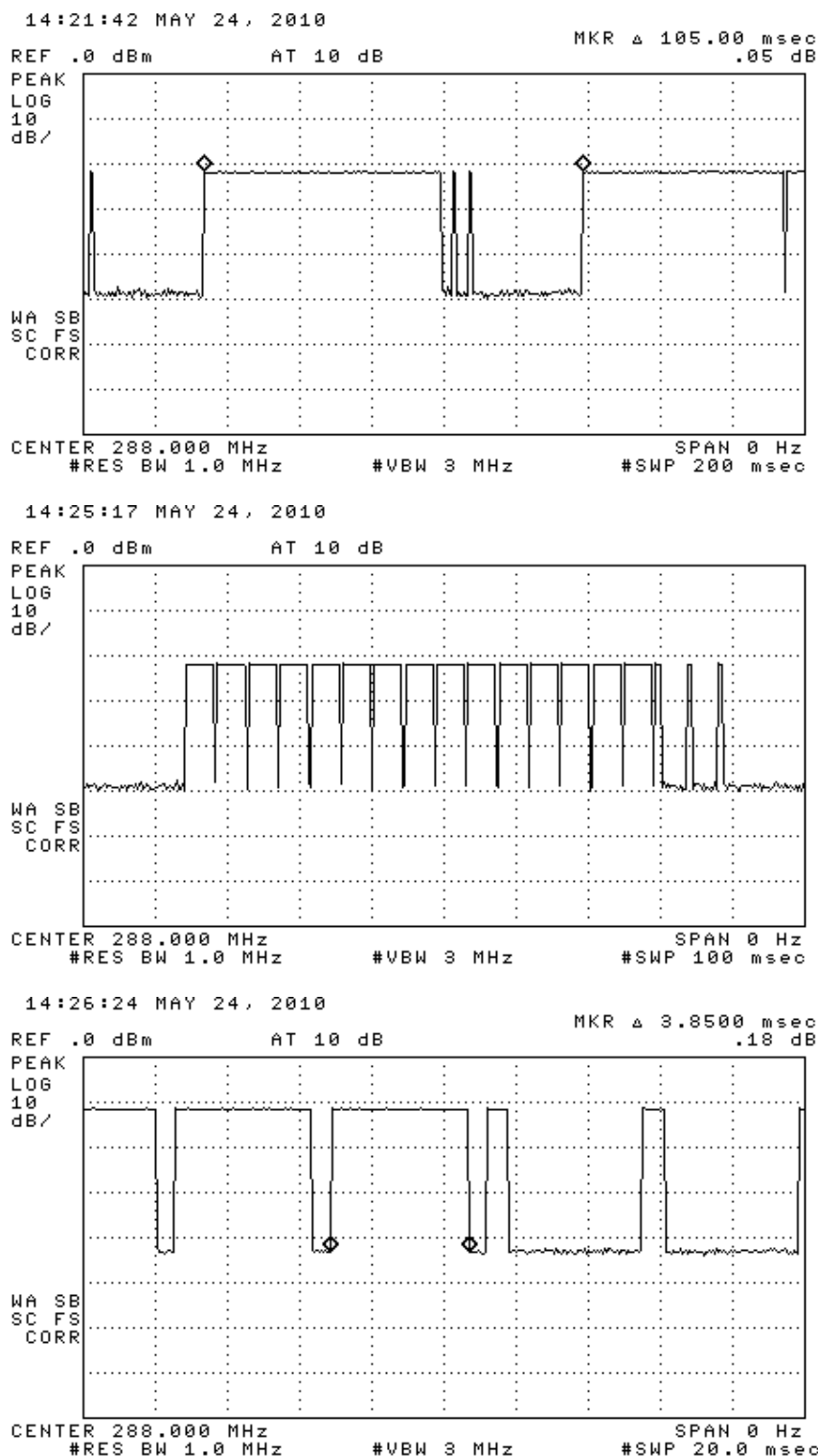
Figure 6.1(g). Transmission modulation characteristics 288 MHz. (top) maximum on time transmission, (center) expanded word, (bottom) PWM bit width.
