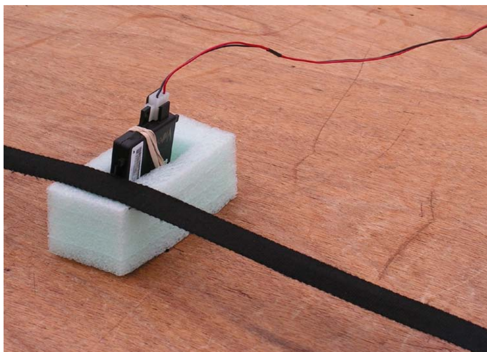
Photograph 6.6. Close-up of DUT on OATS (one of three axes tested)
