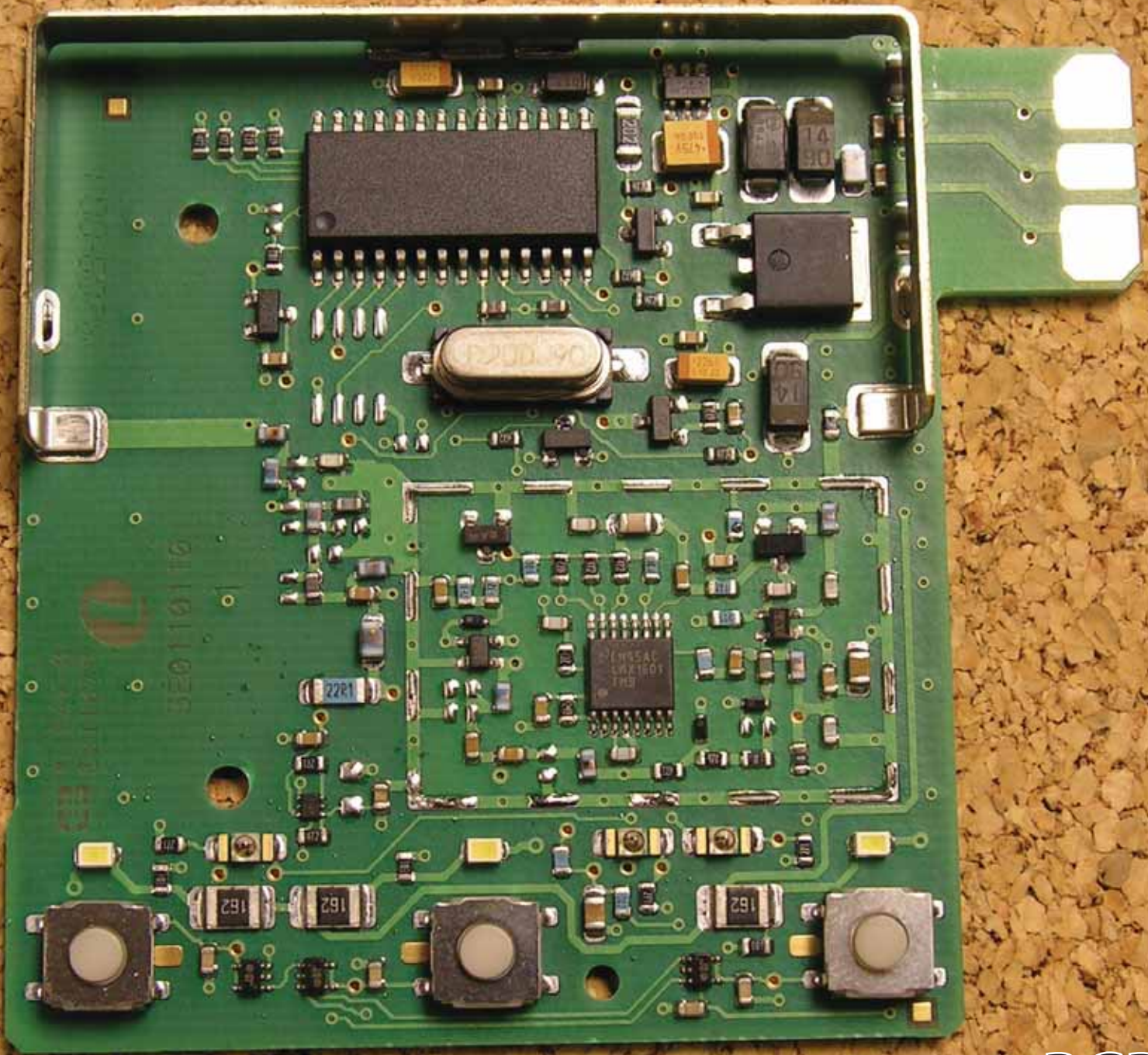
PCB (top)
