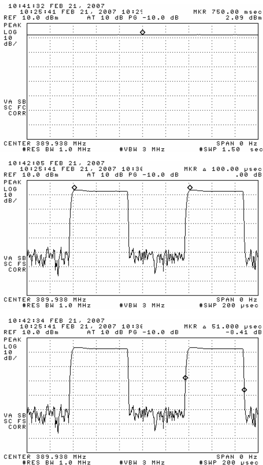
Figure 6.1(c). Transmissions modulation characteristics, 390 MHz: (top) low duty complete transmission, (center) expanded bit, (bottom) expanded period.
