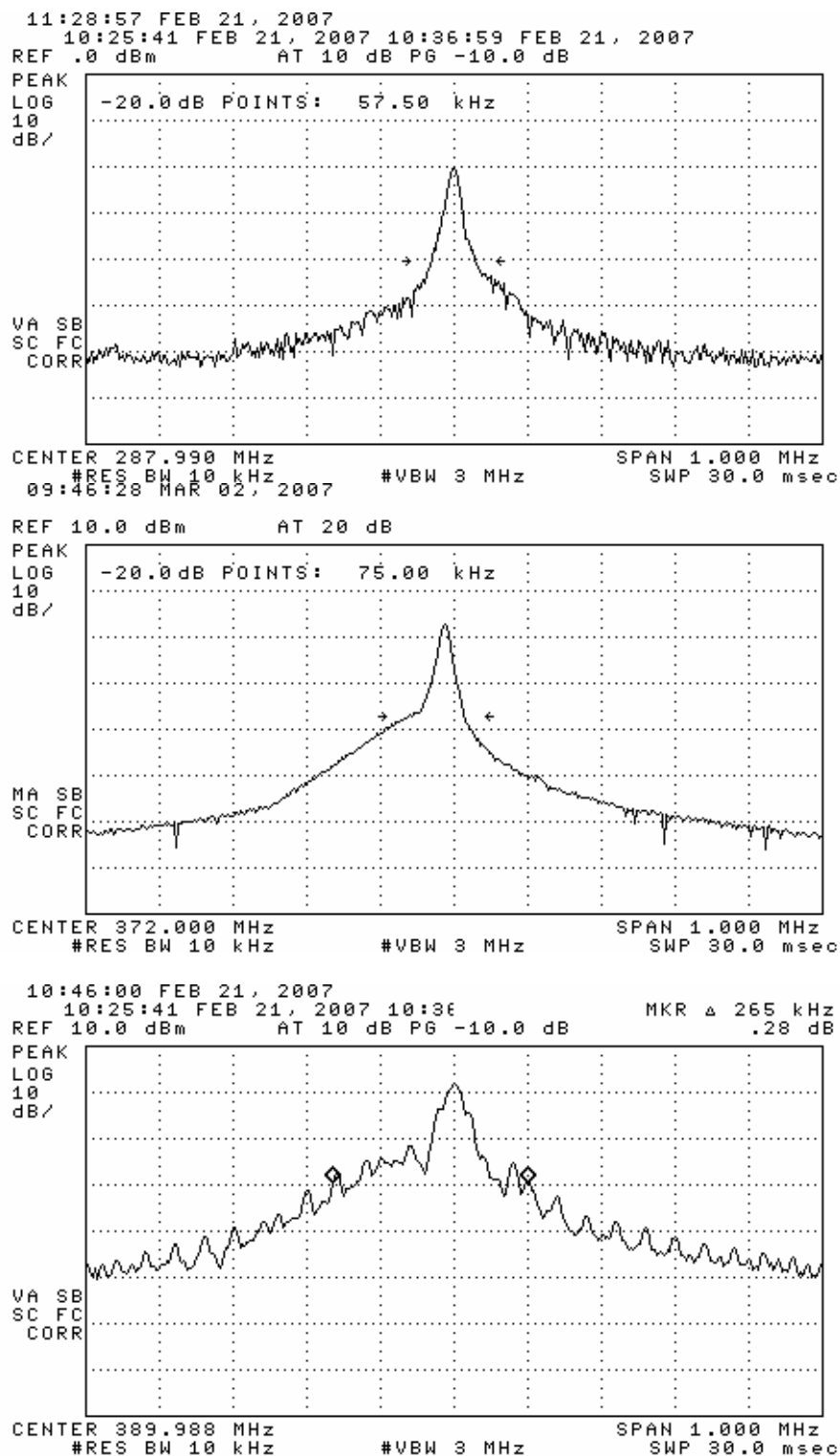
Figure 6.3. Worst case measured bandwidths at select frequencies. (pulsed emission, highest data rate).
