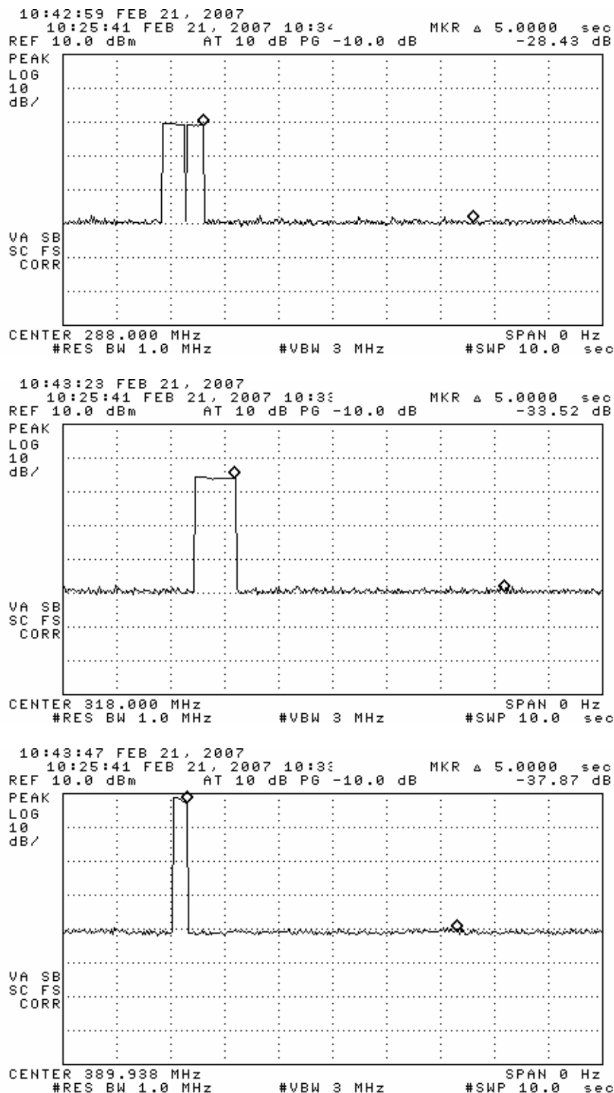
Figure 6.4(a). Transmitter 5 sec. transmission limit verification. (normal operating mode)
