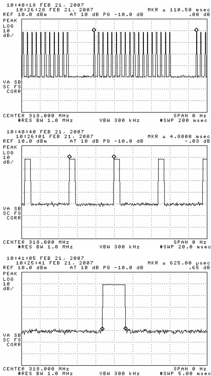
Figure 6.1(b). Transmissions modulation characteristics, 318 MHz: (top) high duty complete transmission, (center) expanded bit, (bottom) expanded period.
