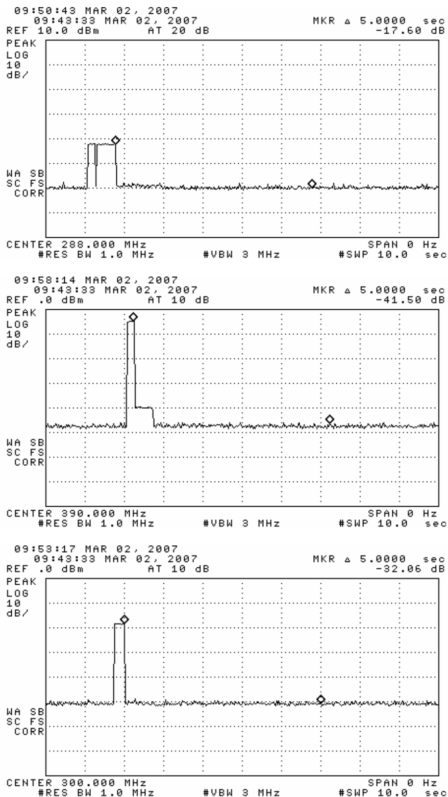
Figure 6.4(b). Transmitter 5 sec. transmission limit verification. (top) 8 dip-switch programming mode (middle) 9 dip-switch programming mode (bottom) 10 dip-switch programming mode
