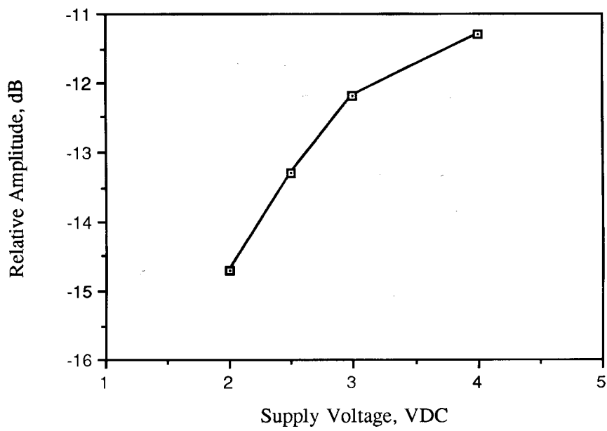
Figure 6.4. Relative emission at 315.0 MHz vs. supply voltage (CW emission).
