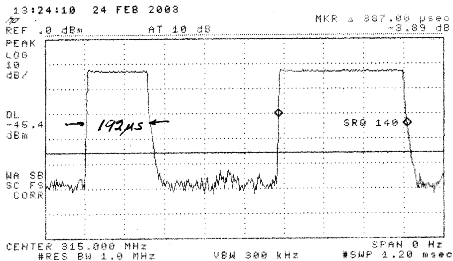
Figure 6.1(cont.). Transmissions modulation characteristics: (top) superhét pre-amble, (center) regen pre-amble, (bottom) expanded bits.
