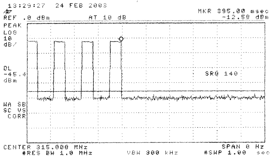
Figure 6.5. Emission after the DUT button is released.
