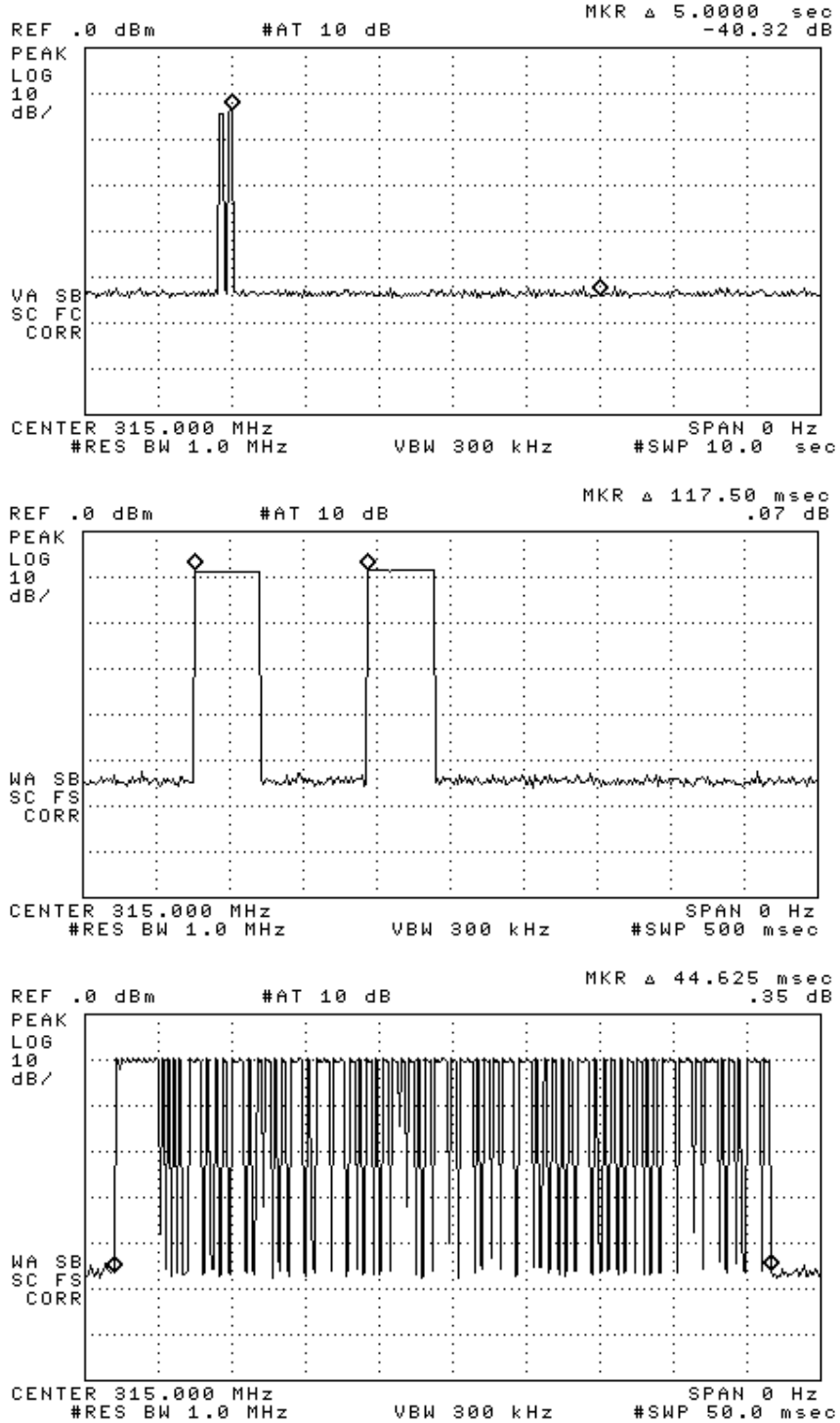
Figure 6.1(a). Transmission modulation characteristics. (top) single manual transmission, (bottom) expanded frame
