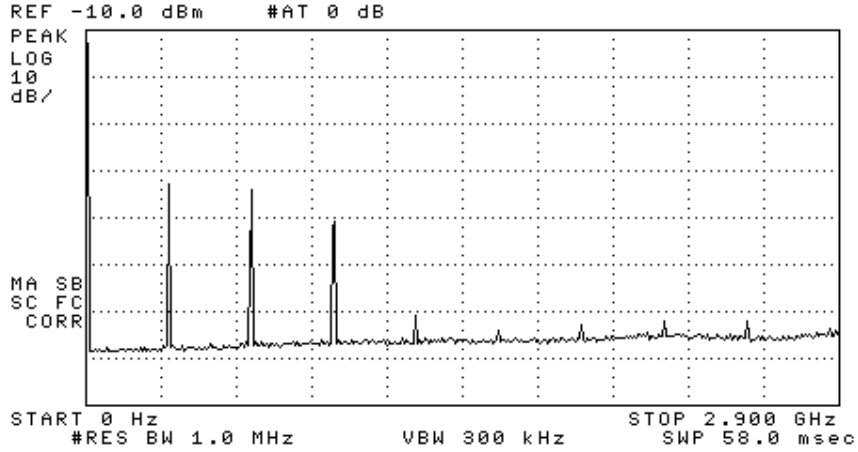
Figure 6.2. Emission spectrum of the DUT (pulsed emission). Amplitudes are only indicative (not calibrated).
