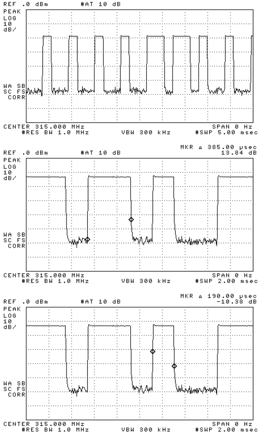
Figure 6.1(b). Transmission modulation characteristics. (top) PWM frame encoding, (center) PWM wide, (bottom) PWM narrow.
