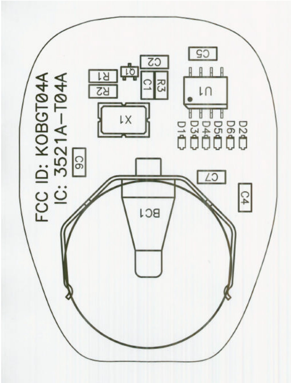
Figure 1. Bottom side component layout of GM RFA04 Transmitter
