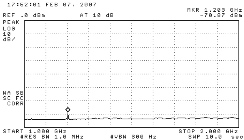
Figure 5.2. Emissions measured at 3 meters in chamber, 1000-2000 MHz. (emission at marker is background) (top) Internal Antenna, (bottom) External Antenna
