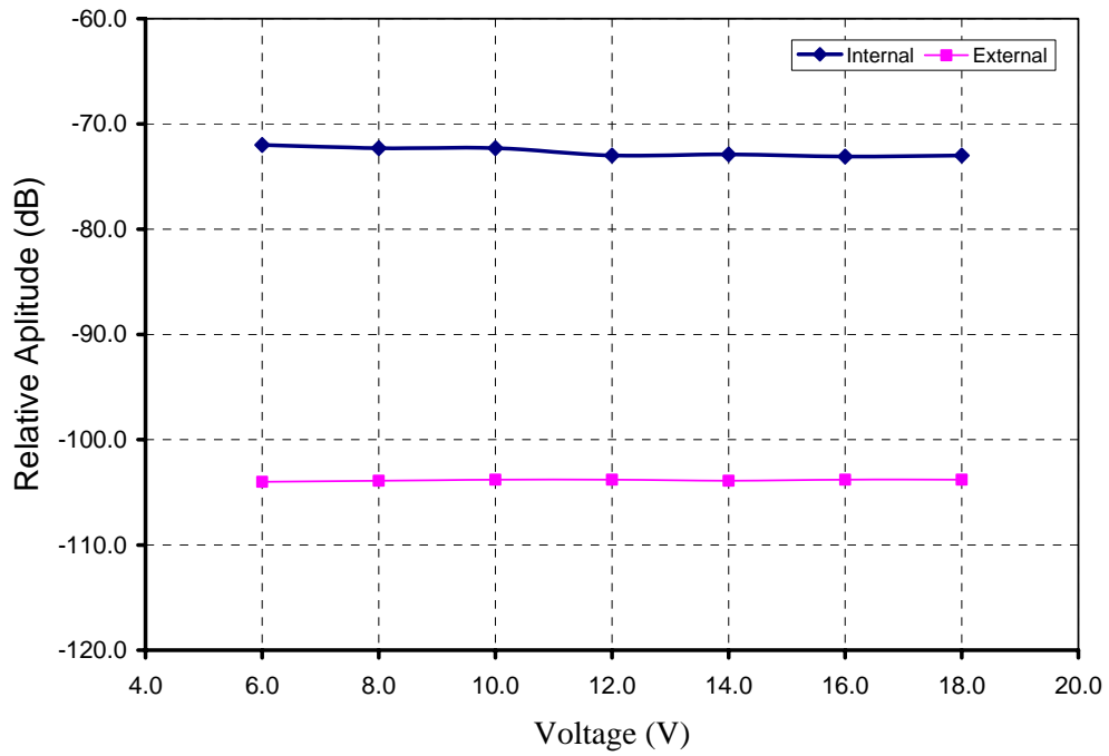
Figure 6.2. Relative emission at vs. supply voltage.
