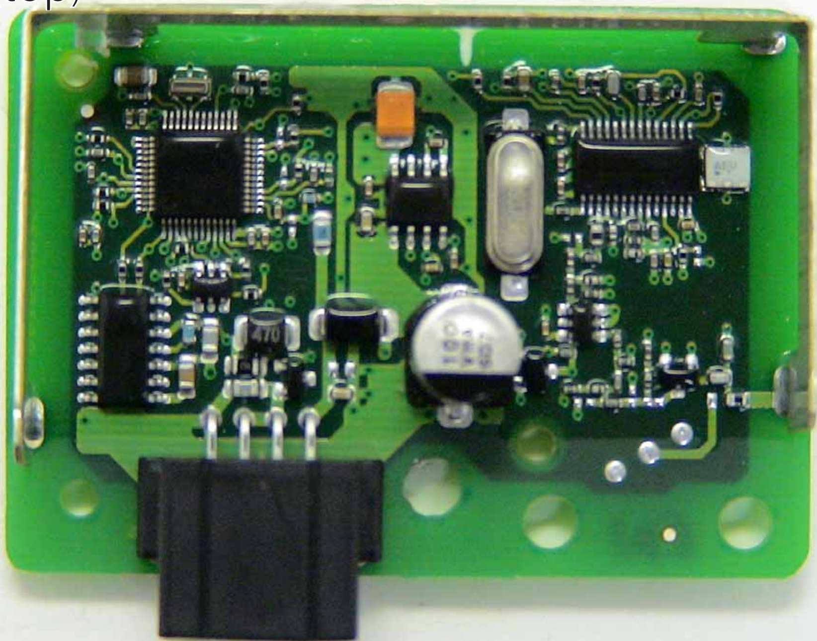
PCB (top)
