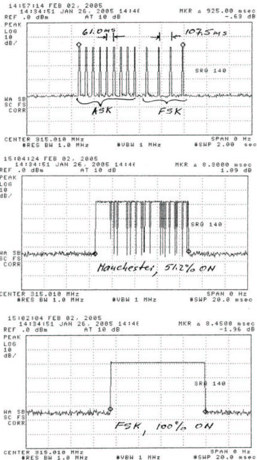
Figure 6.1. Transmissions modulation characteristics: (top) complete transmission, (center) expanded ASK, (bottom) expanded FSK.
