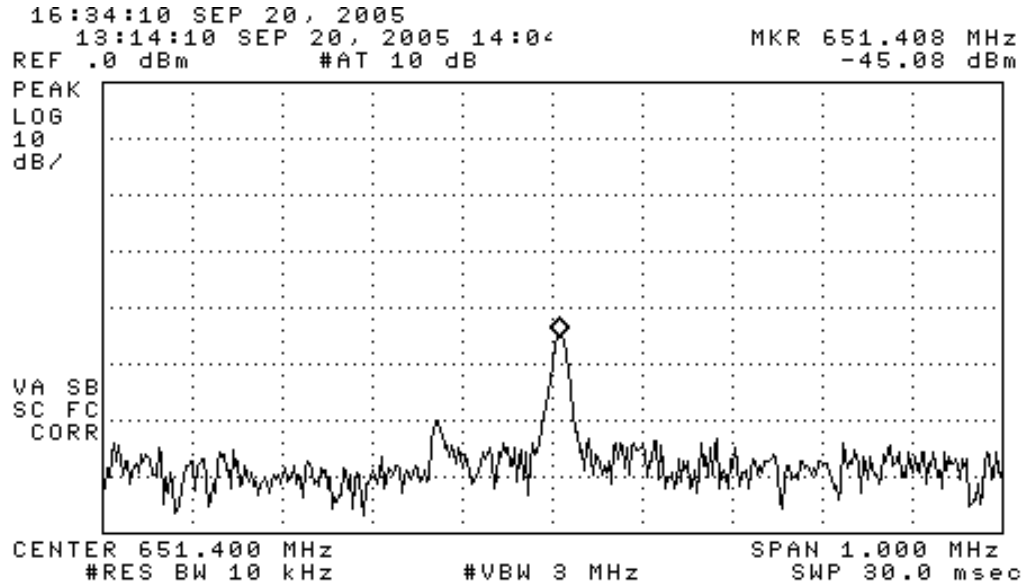
Figure 6.1. Relative receiver emissions (40 dB Amplifier Gain not included).
