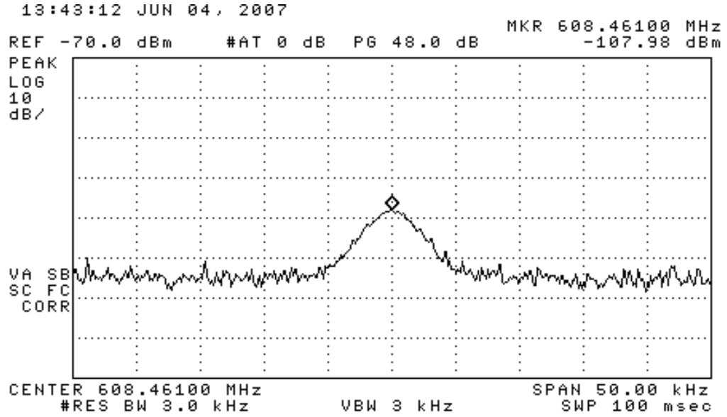
Figure 6.1. Relative receiver emissions (2 x LO).
