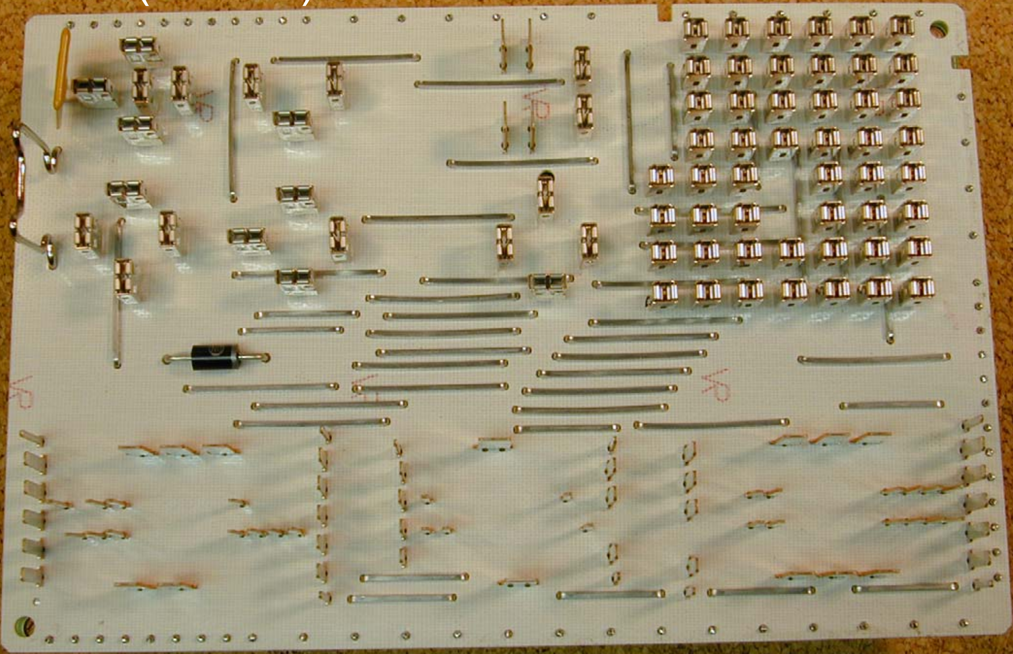
PCB 1 (bottom)
