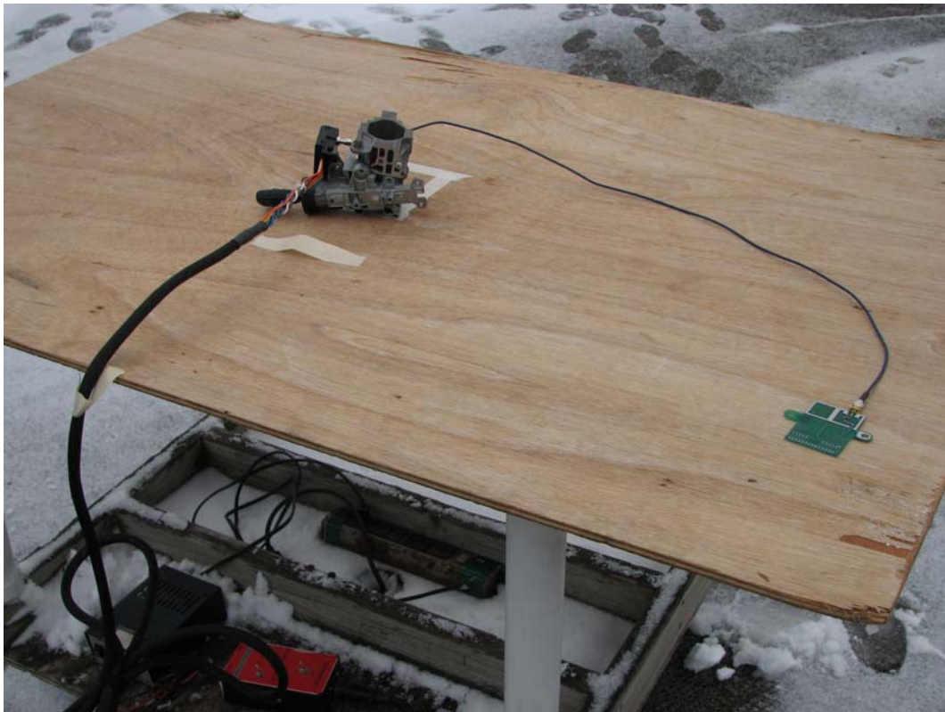
DUT (05E01H01) on OATS (close-up)
