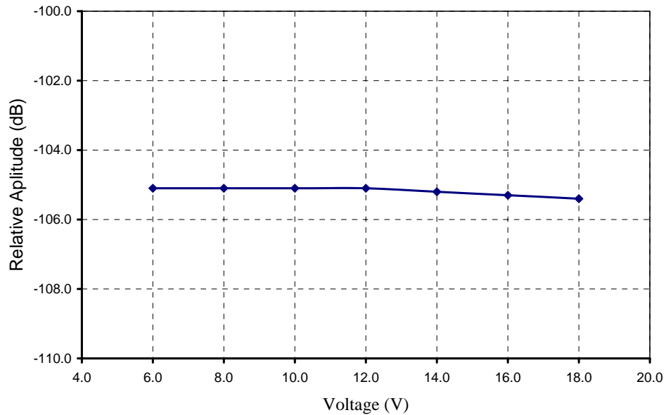
Figure 6.2. Relative emission vs. supply voltage.
