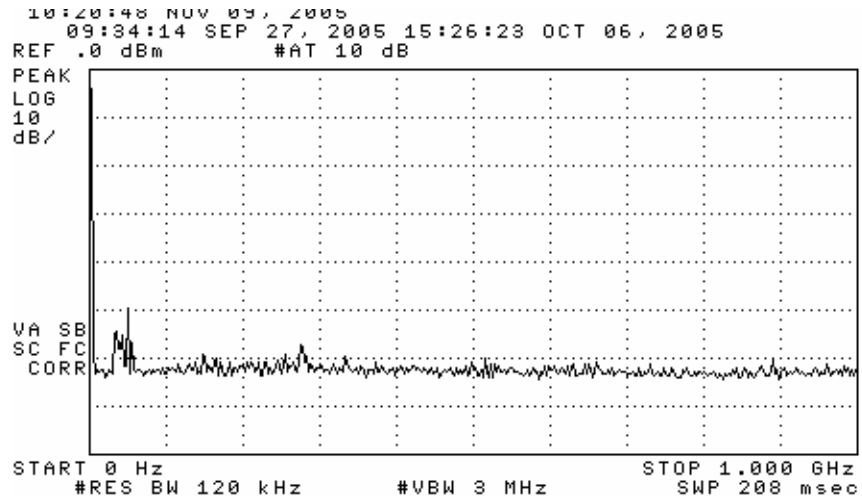
Figure 5.1. Emissions measured at 3 meters in chamber, 0-1000 MHz.
