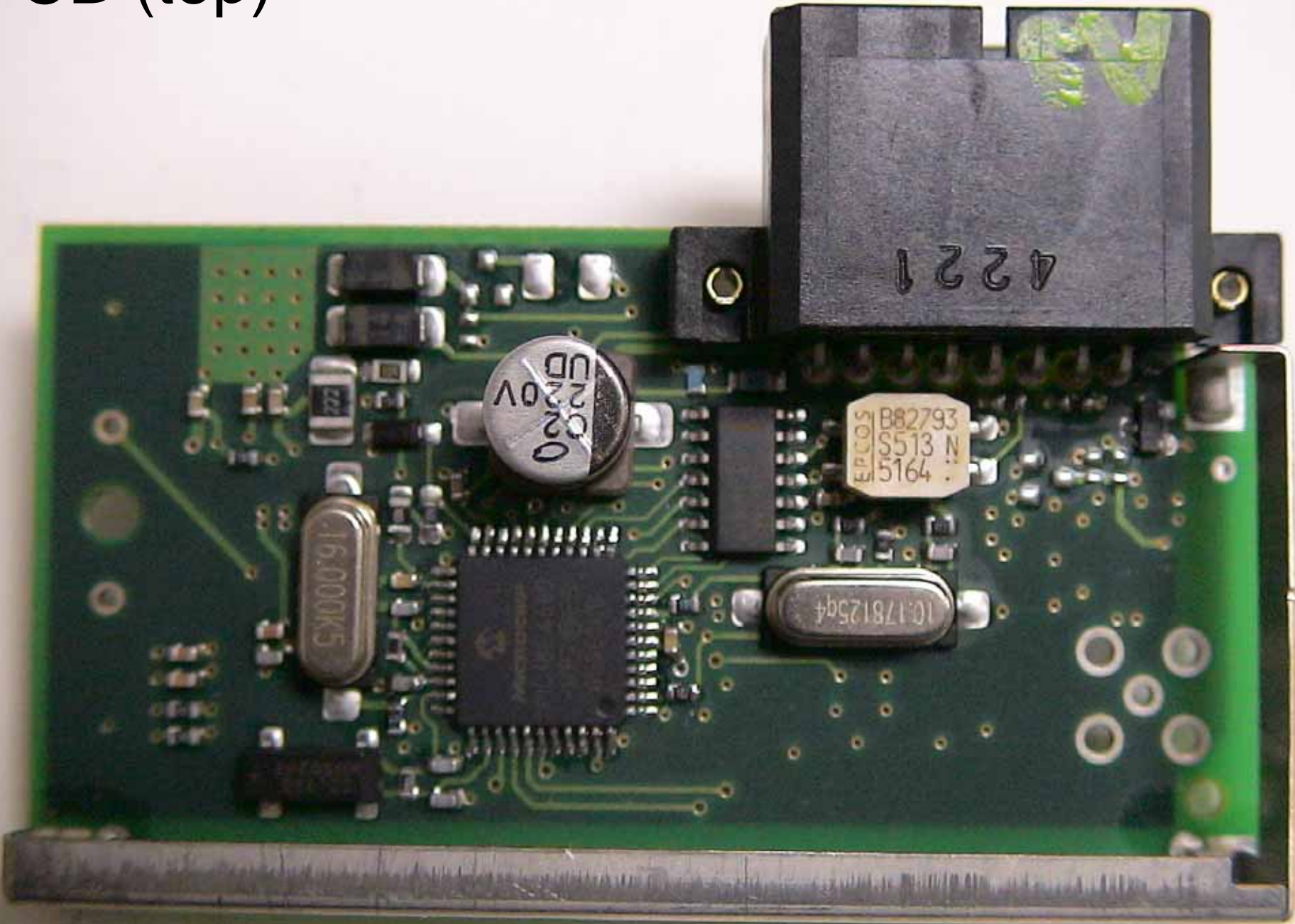
PCB (top)
