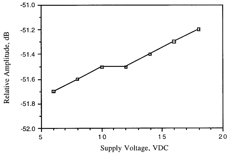
Figure 6.2. Relative emission at 651.4 MHz vs. supply voltage.
