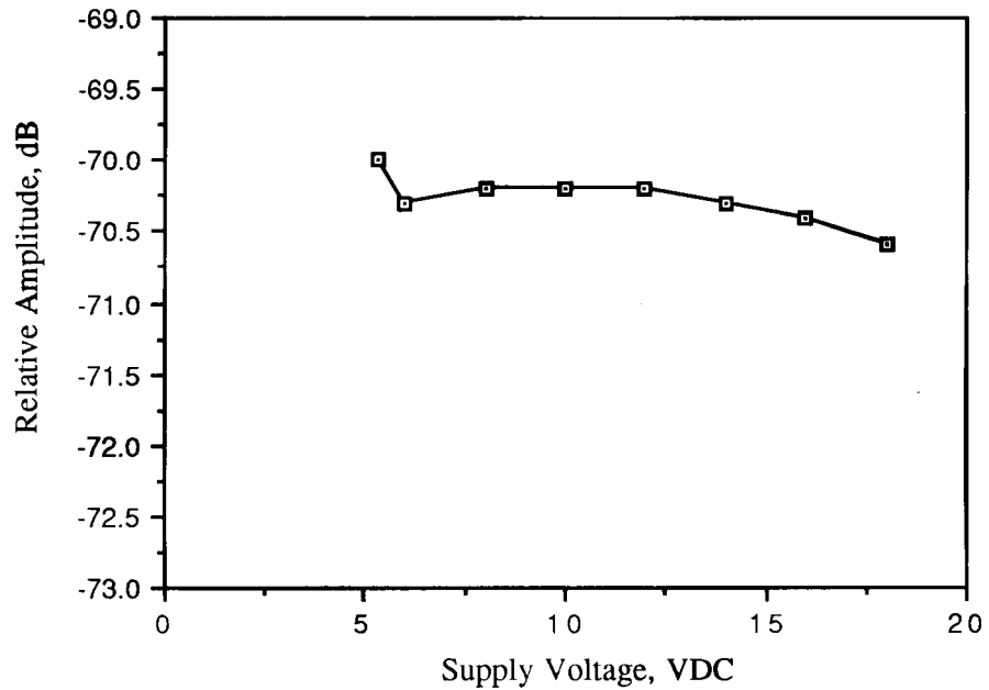
Figure 6.2. Relative emission at 651.4 MHz vs. supply voltage.
