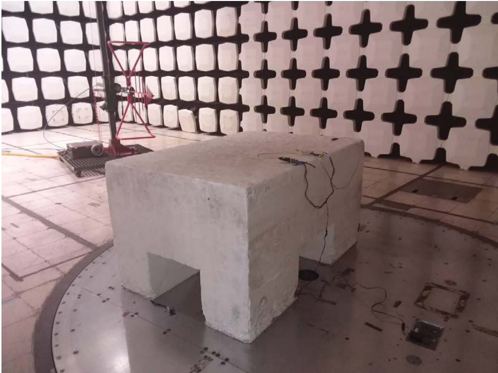
Radiated Emissions
